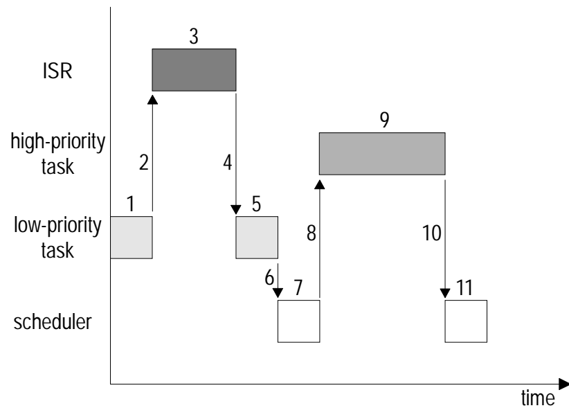
Figure 4: Cooperative Scheduling
