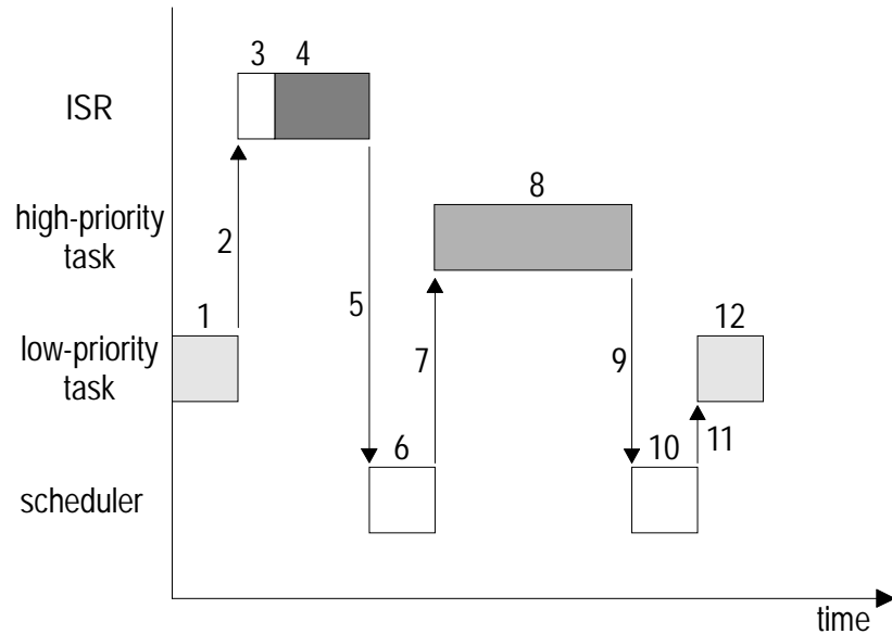
Figure 3: Preemptive Scheduling
