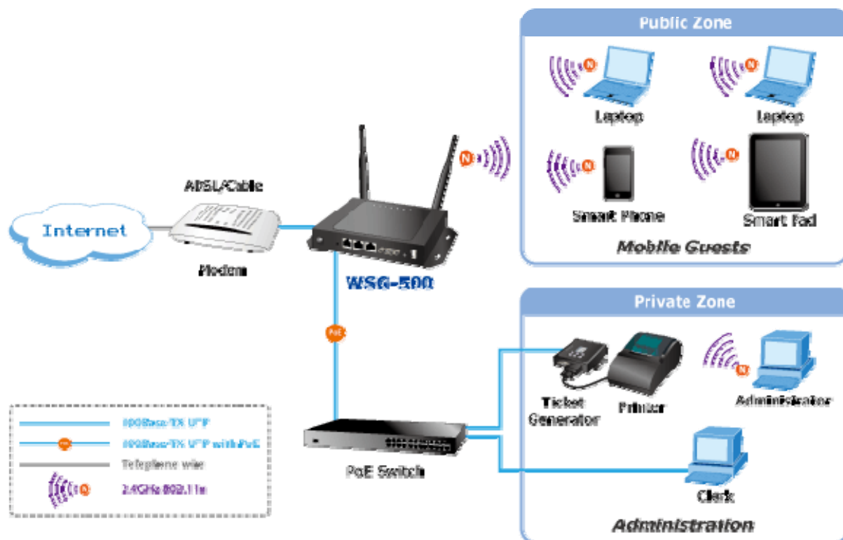
[Example: A typical Hotspot network]
