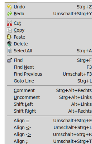
Figure 4: Edit menu
