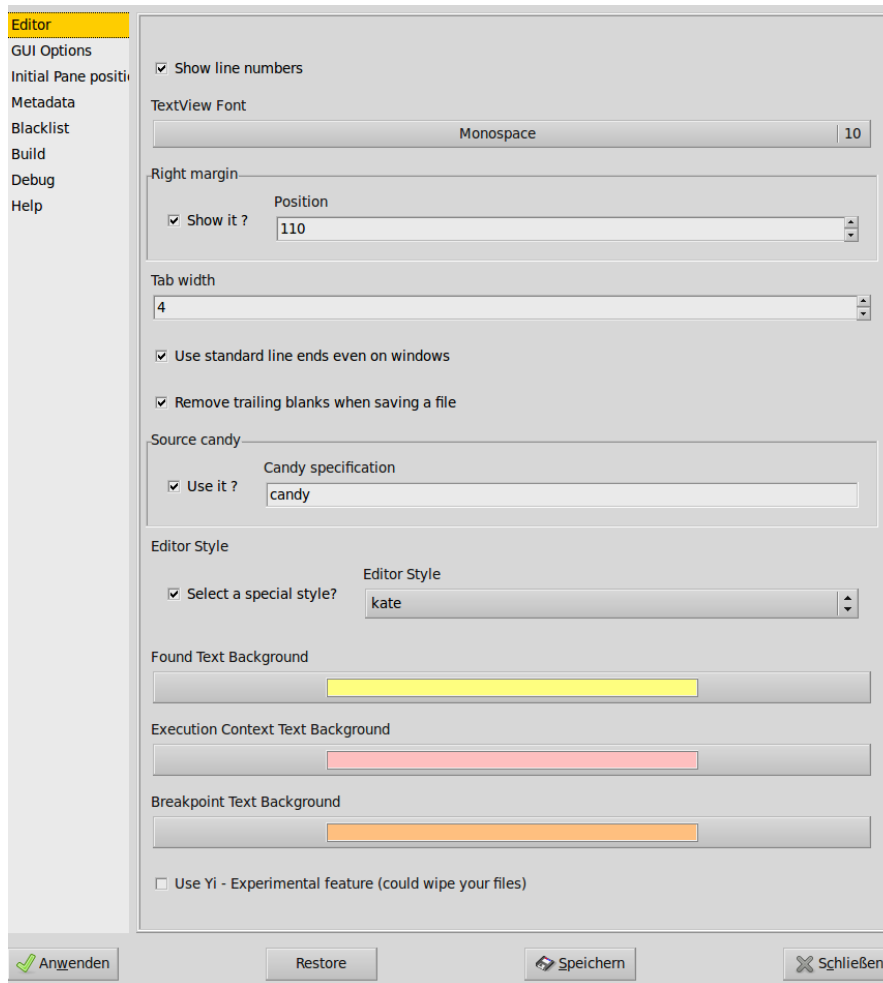
Figure 9: Editor Preferences
