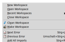
Figure 10: Workspace Menu
