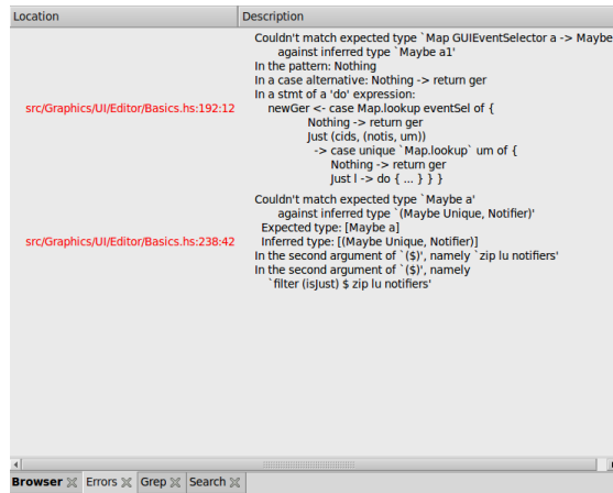
Figure 13: Error Pane
