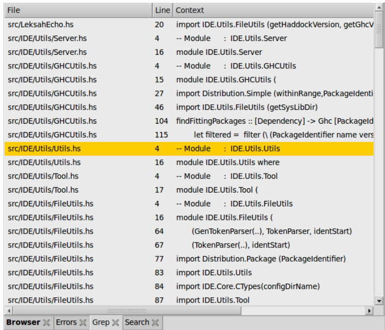
Figure 6: Grep pane
