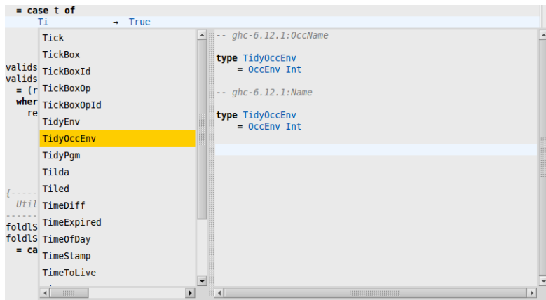
Figure 8: Completion
