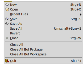
Figure 3: File menu
