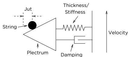
Figure 25: Second pick model
