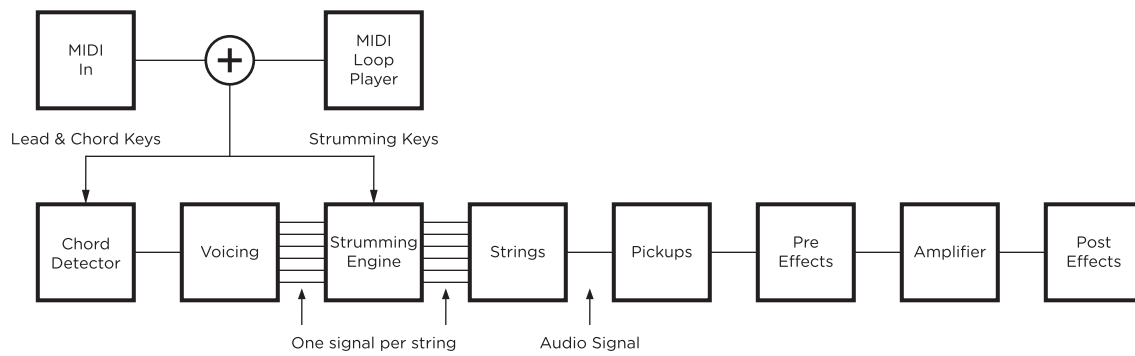
Figure 9: General architecture of Strum .
