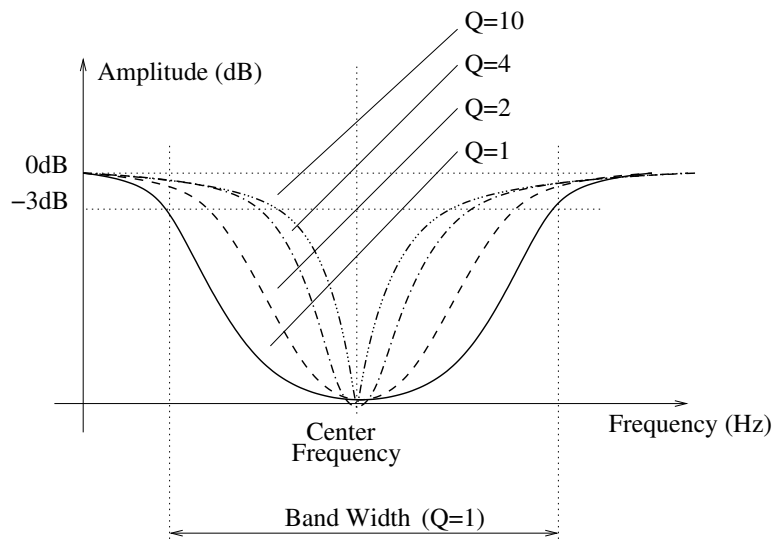
Figure 22: Frequency response of a notch filter.
