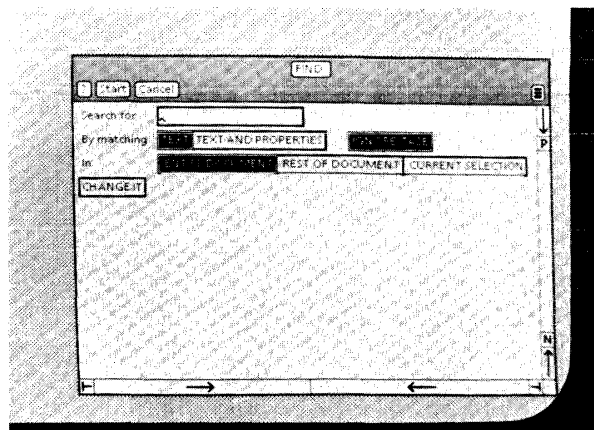
Figure 17—The option sheet for the Find command
