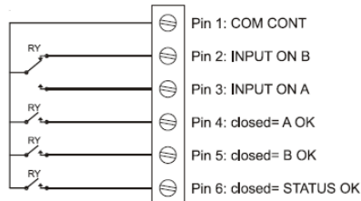
Fig. 2: Contacts port basic diagram.
