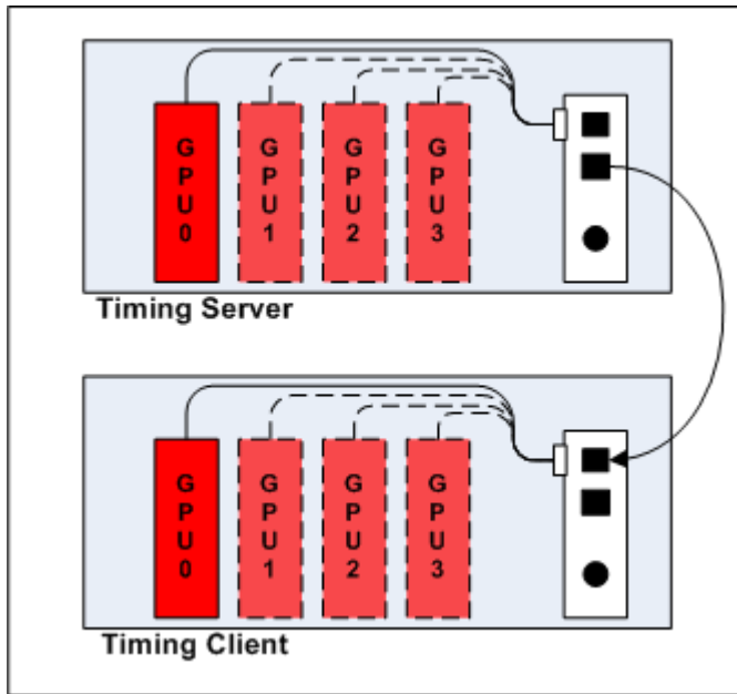
Figure 6-4 Two PCs with Four GPUs Each Framelocked
