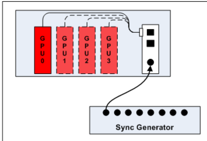
Figure 6–2 Single PC with Four GPUs Genlocked to an External Signal Generator
