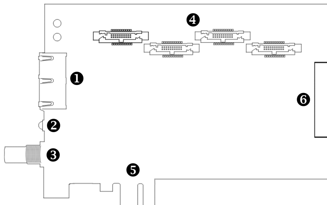
Figure 6–1 ATI FirePro S400 Side View
