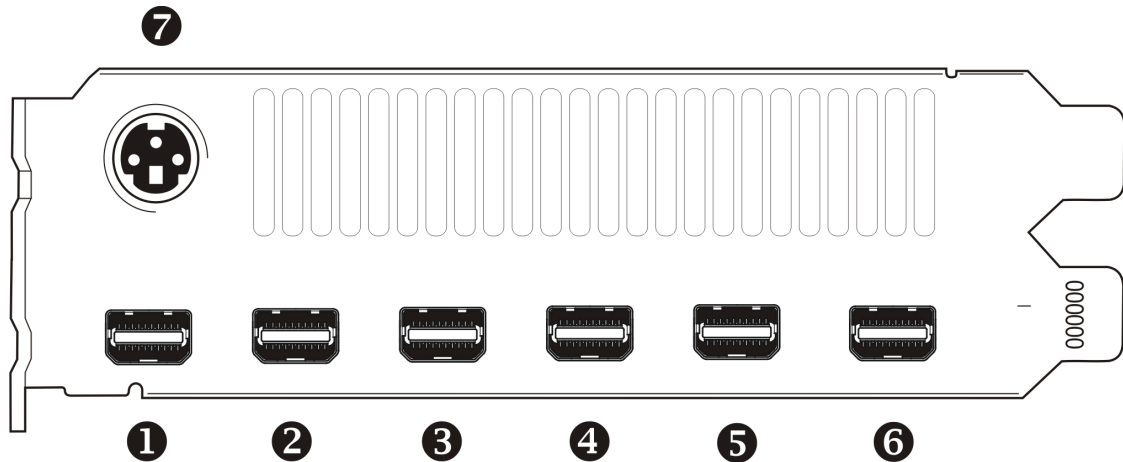
Figure 3-1 AMD FirePro™ W9000 Baseplate Connections
