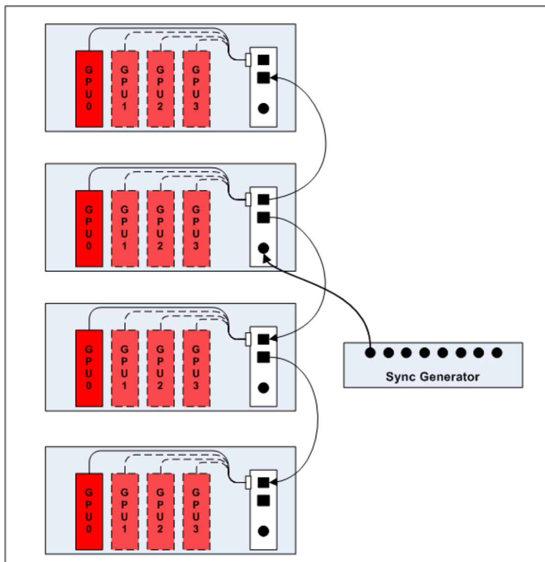
Figure 6–5 Four PCs Framelocked and Genlocked
