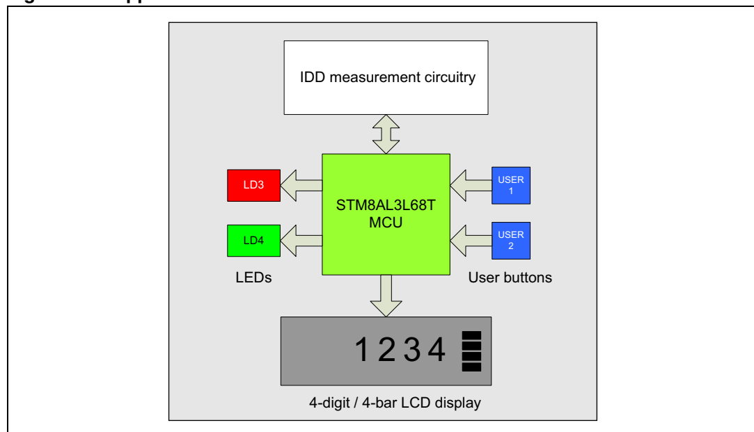
Figure 1. Application schematics
