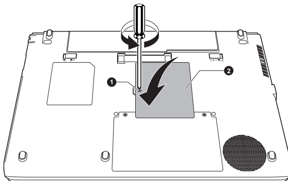
Figure 4-13 Seating the memory module cover (R940)
