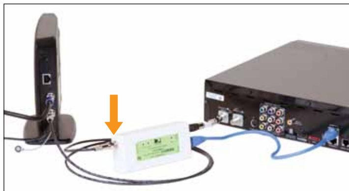
Connect Enclosed Coaxial Cable to "Towards LNB" on the Connected Home Adapter
