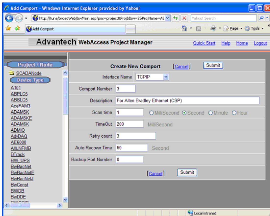
Figure 3.1 TCP/IP Comport properties for Allen-Bradley AB Ethernet to PLC5E, typical settings
