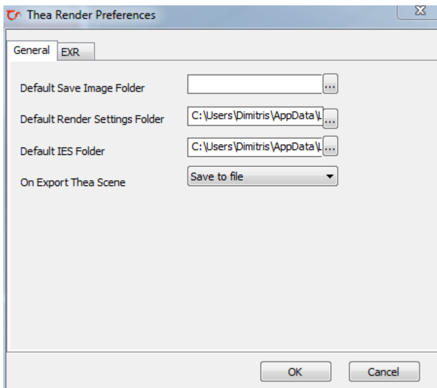
Figure 23: General settings
