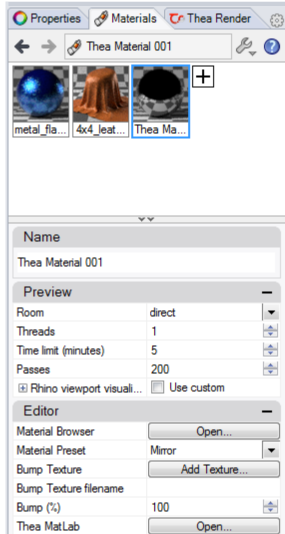
Figure 15: Material section
