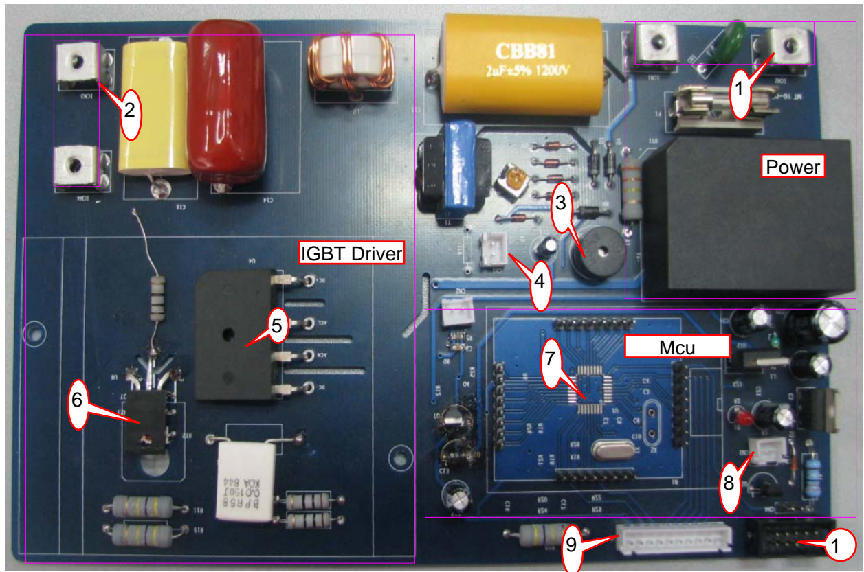
Figure 4-3: Main Board
