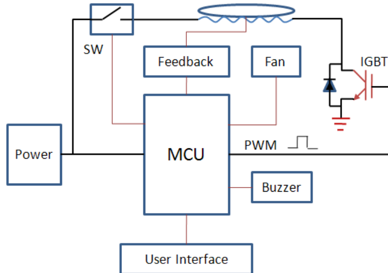
Figure 3-1: Hardware Block Diagram
