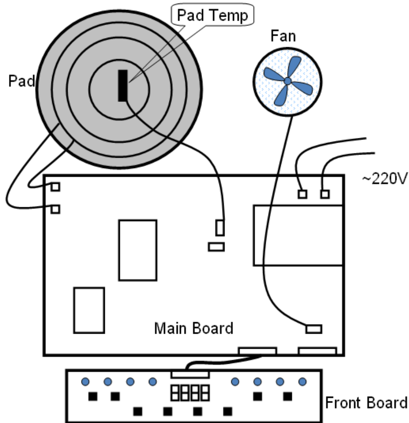
Figure 4-1: System Connection Diagram
