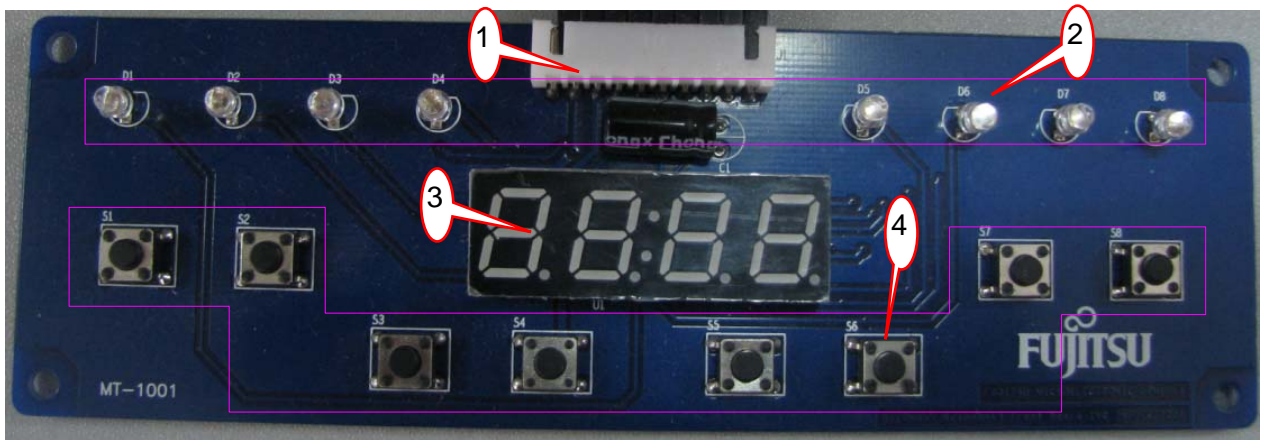
Figure 4-2: Front Board
