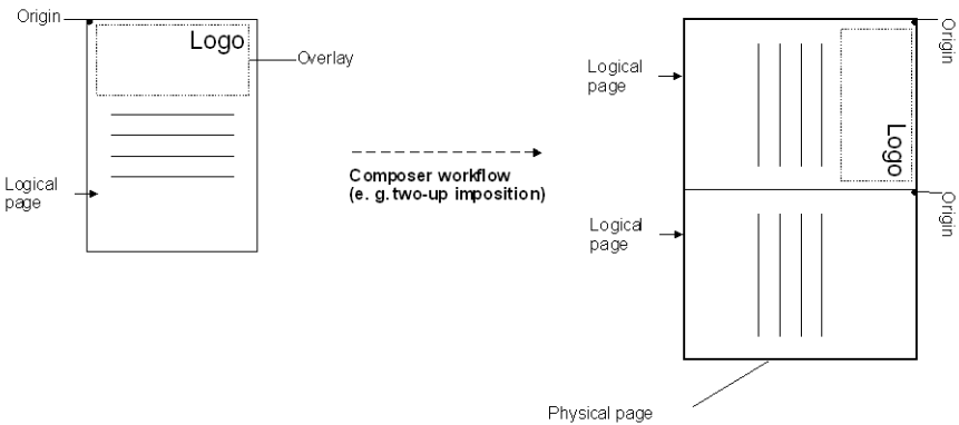
Figure 4 Static linking of the overlay with a logical page.
