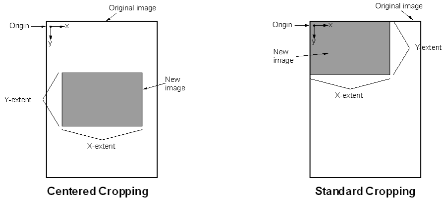
Figure 13 Comparison between 'centred cropping' and 'standard cropping'
