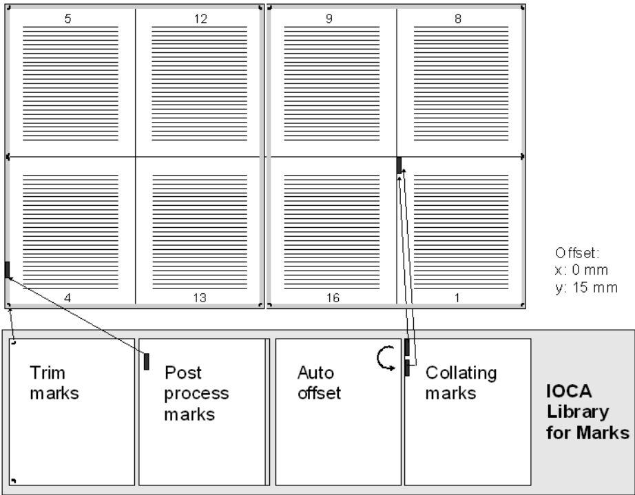
Figure 66 Inserting marks in the print file
