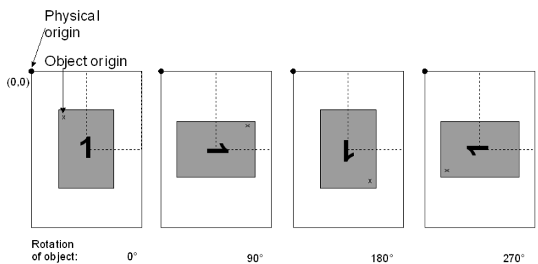
Figure 49 Positioning with "One Up" and 'centred print'
