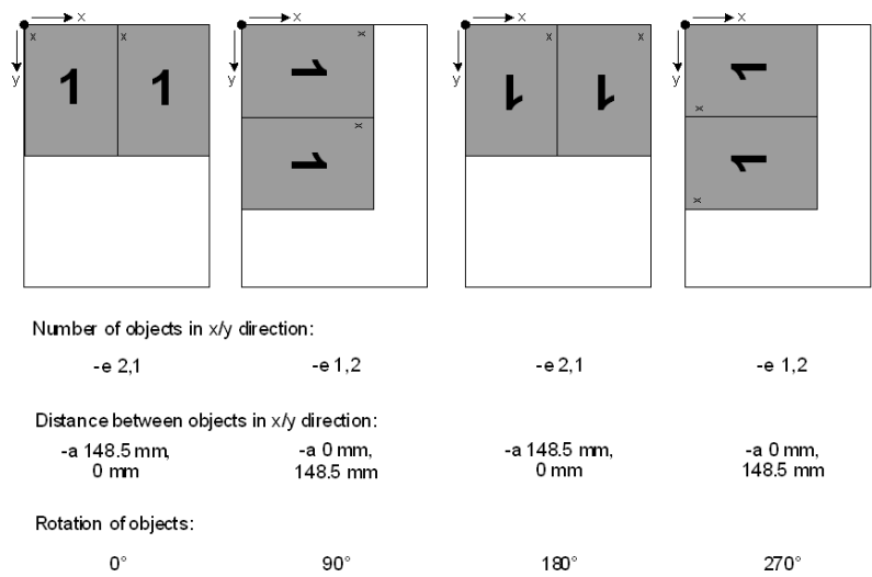
Figure 46 Positioning of 2 A5 objects on A3 paper with various rotations (up to version 4.0)
