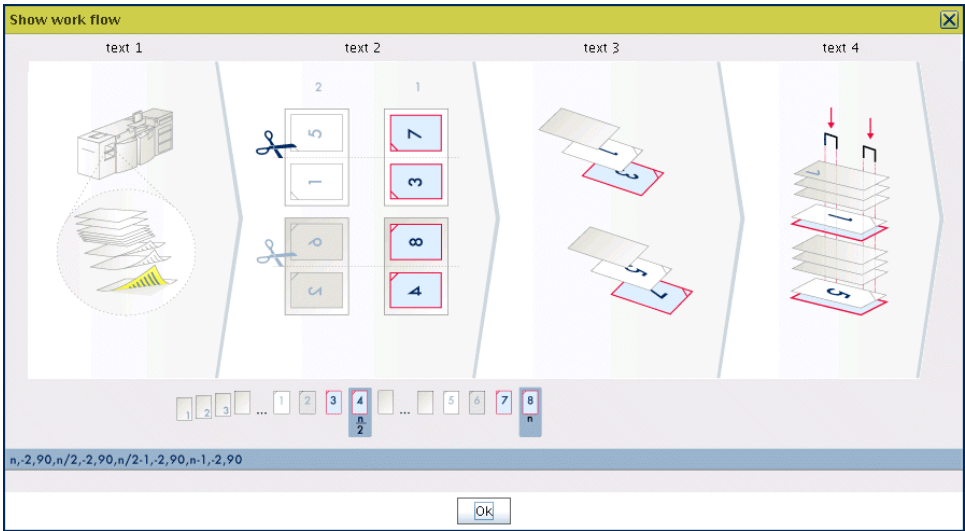
Figure 29 Window 'Impose' – 'work flow': Scheme1, two-up.
