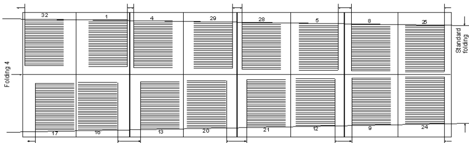
Figure 64 Example for page positioning with 'Signature folding'
