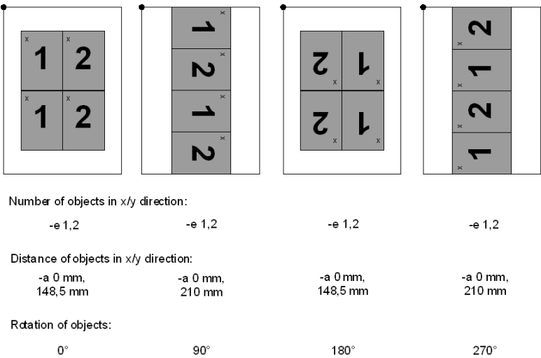
Figure 54 Positioning with "Two Up & Identical copies" and 'centred print'
