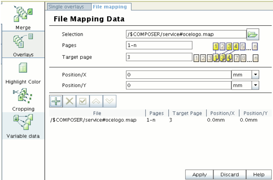
Figure 8 Window 'Overlays' - 'File mapping'
