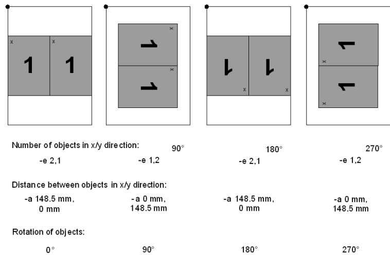
Figure 53 Positioning with "Identical copies" and 'centred print'
