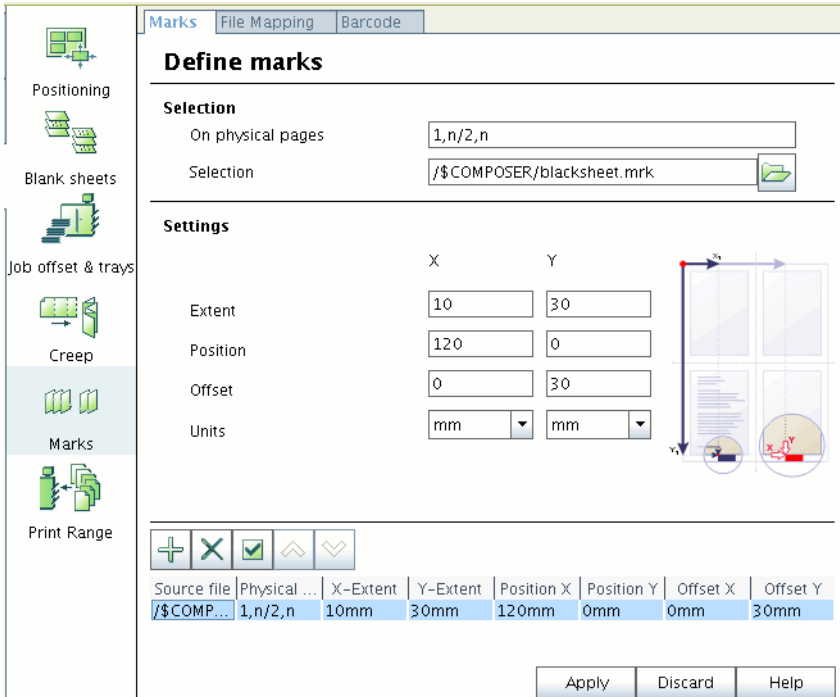
Figure 65 Window 'Marks' - Marks on a single page
