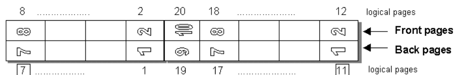
Figure 74 Printed sheets at a range 7 to 11
