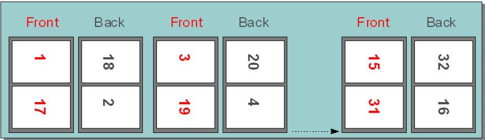
Figure 24 Example file with 32 pages (Two Up, Duplex)
