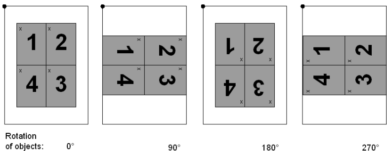
Figure 52 Positioning at "Four Up" with 'centred print'
