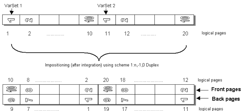
Figure 72 Print file before and after Impositioning "One Up, scheme 2": (n,-1,0), Duplex
