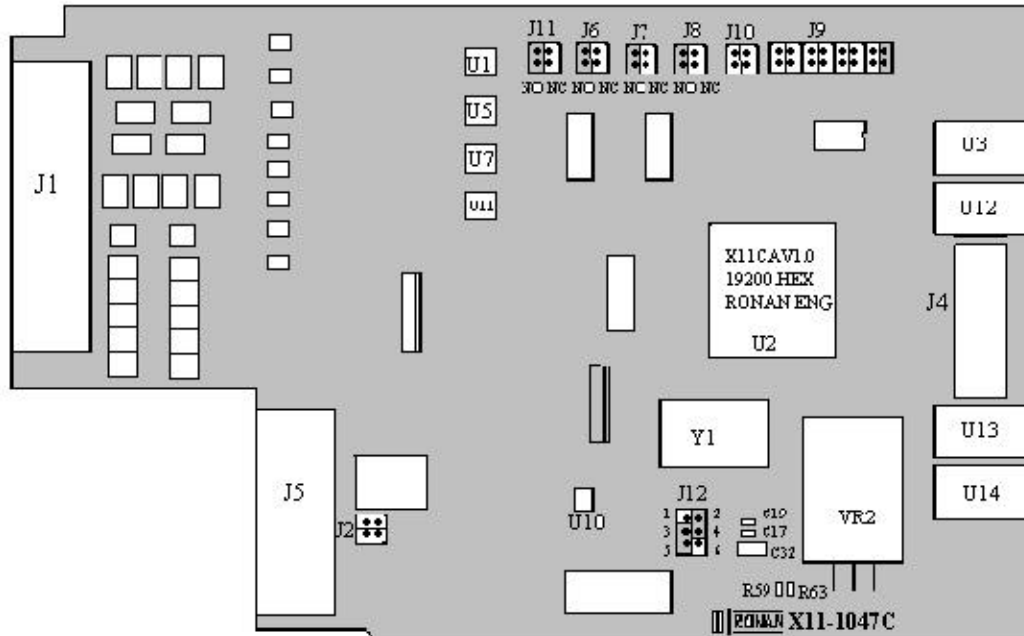
Figure 2-7 X11-1047C Module
