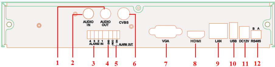
Fig 2-3 Rear Panel for 4-ch
