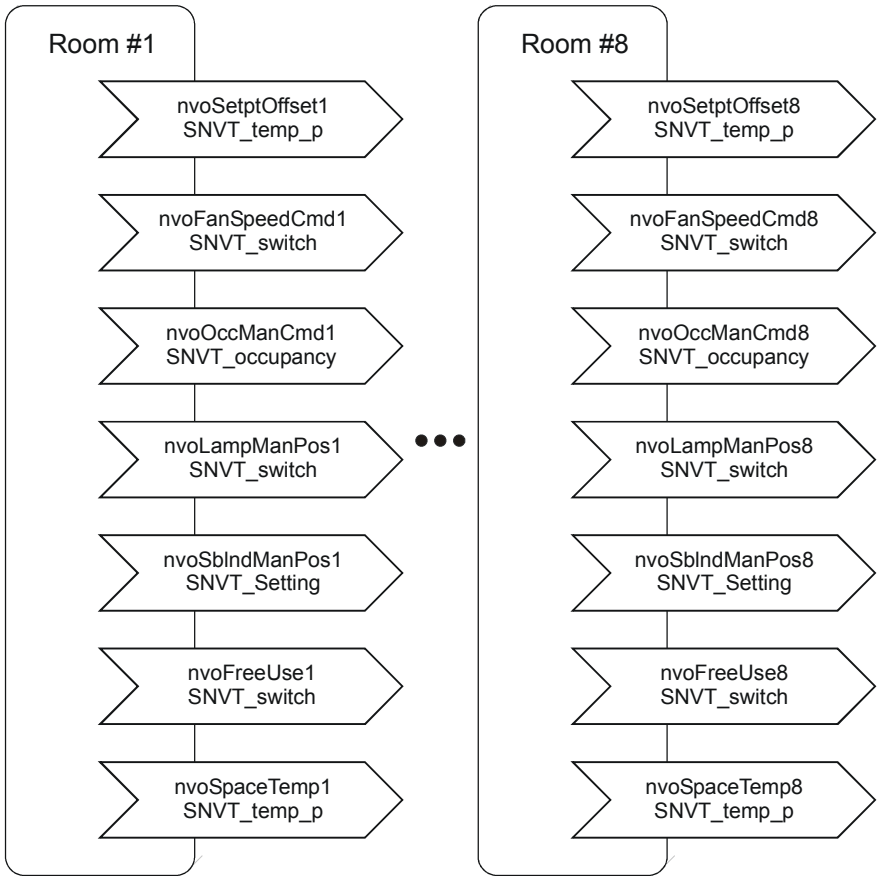
Fig. 16. Network Variables per room
