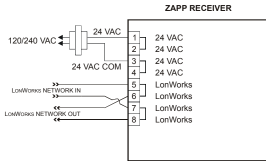
Fig. 3. W7070A terminal assignments
