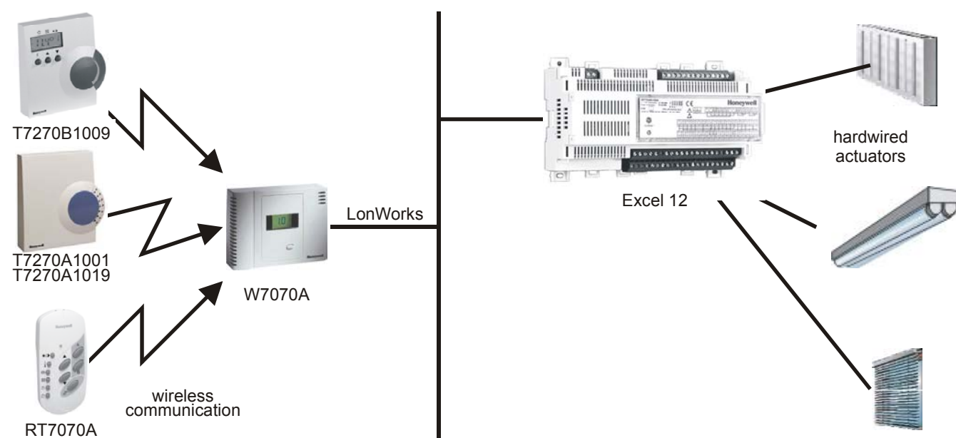
Fig. 1. System overview
