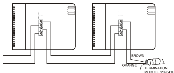
Fig. 2. Termination module connection (daisy-chain network configuration)
