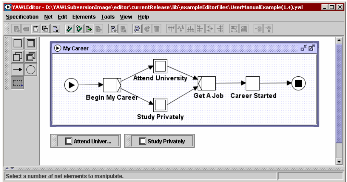
Fig. 15 - Making the "Study Privately " task atomic
