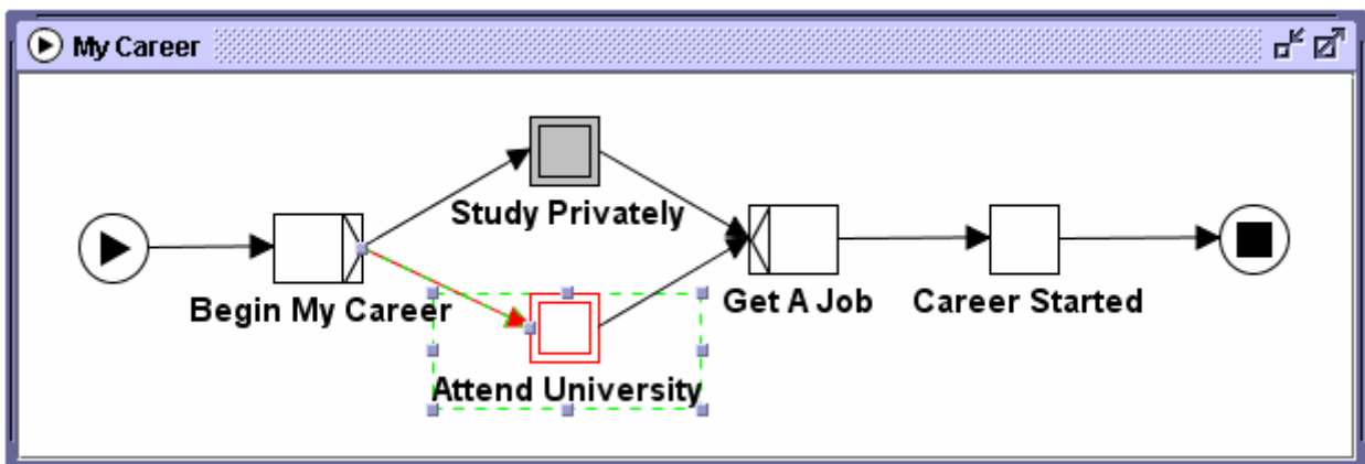
Fig. 20. Adding elements to a Cancellation Set
