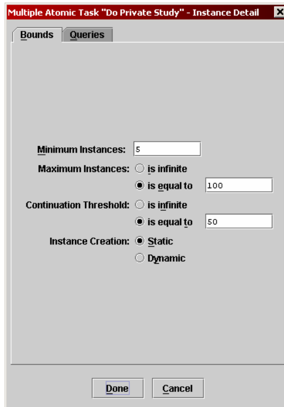
Fig. 11. Instance Bounds on Multiple Instance Tasks
