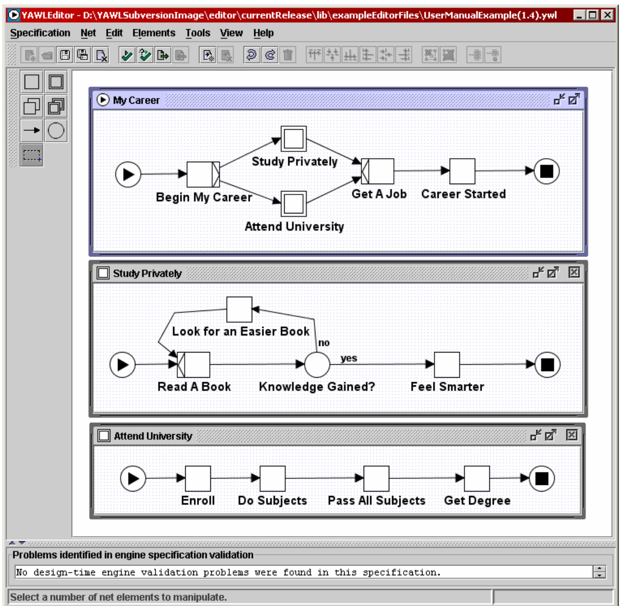
Fig. 35 - The completed scenario specification
