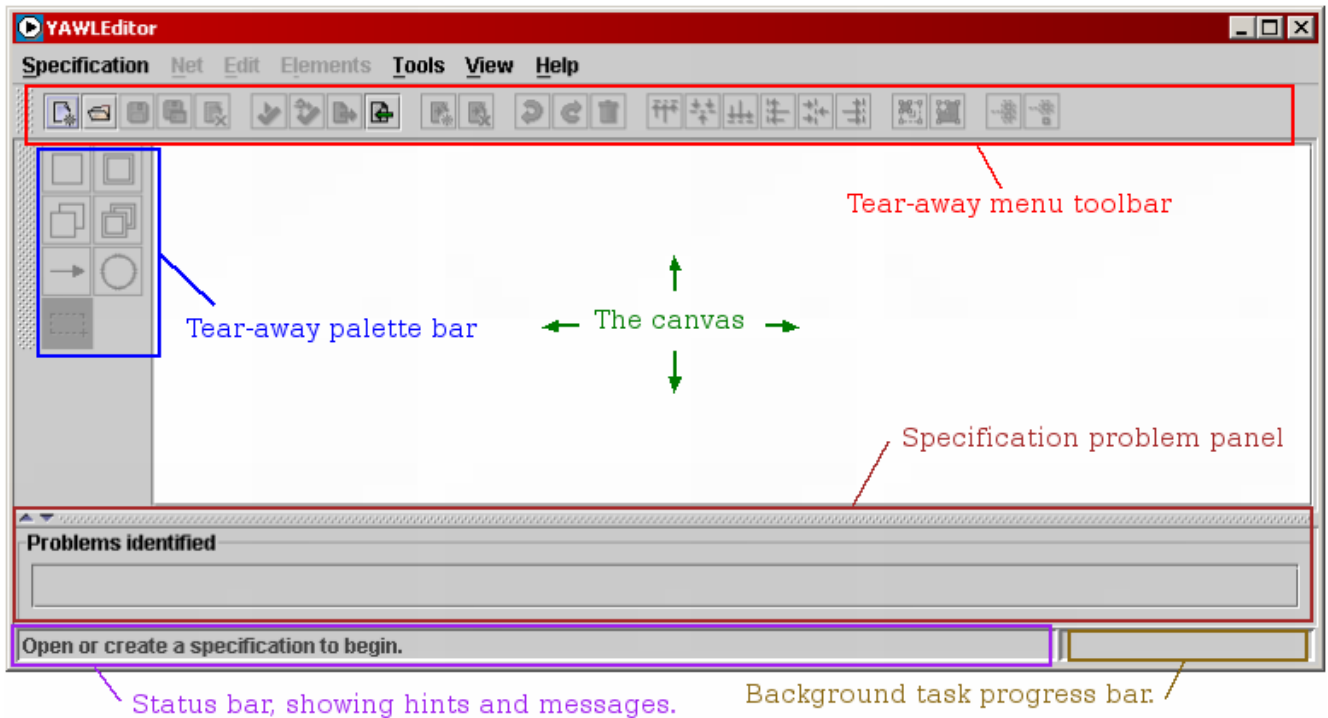
Fig. 2. The YAWLEditor Workspace
