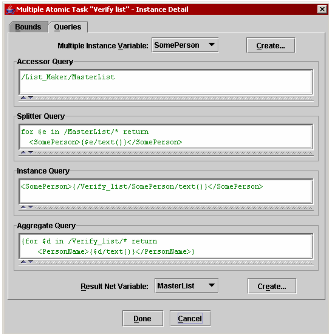
Fig. 44 – Example multiple instance queries
