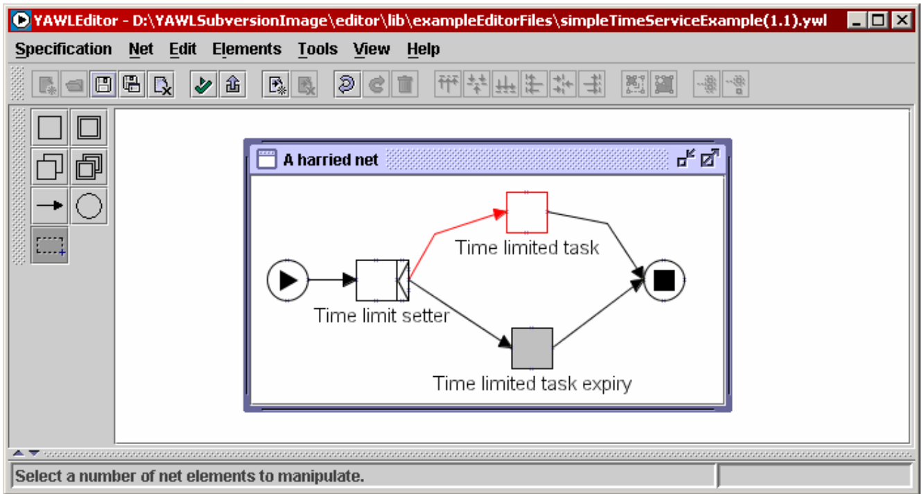
Fig. 45 - Example showing the usage of a custom YAWL service
