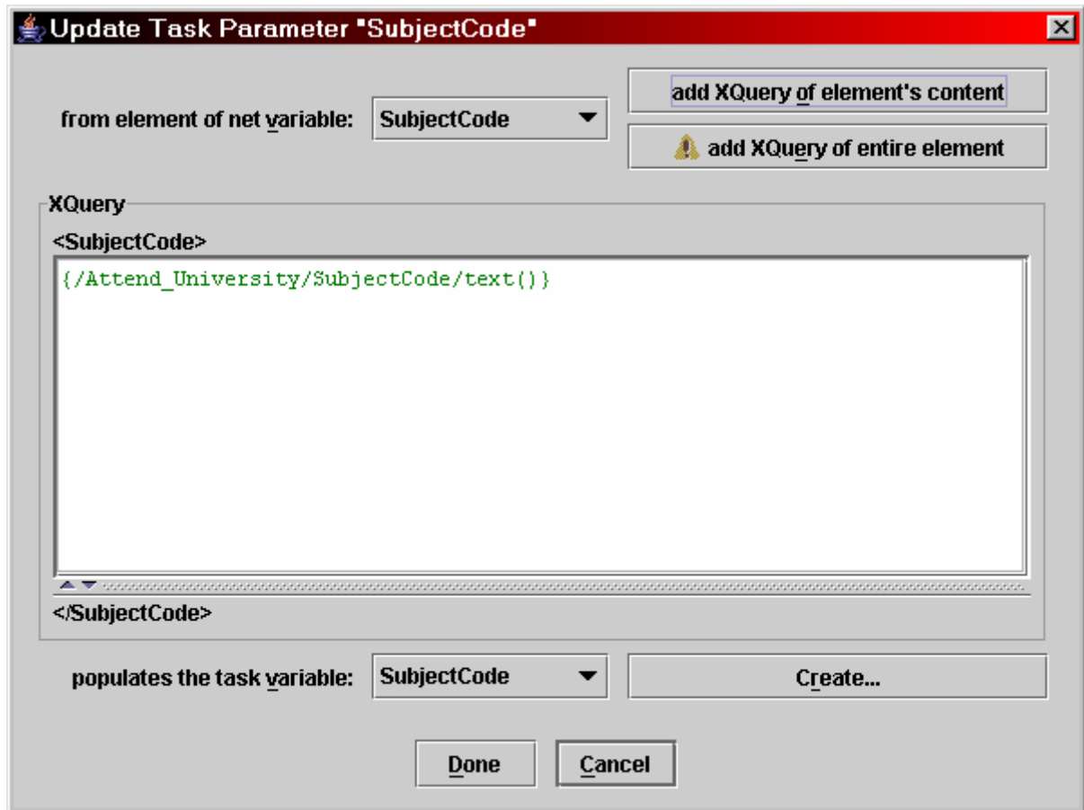
Fig. 32. Passing a net's SubjectCode to a Task
