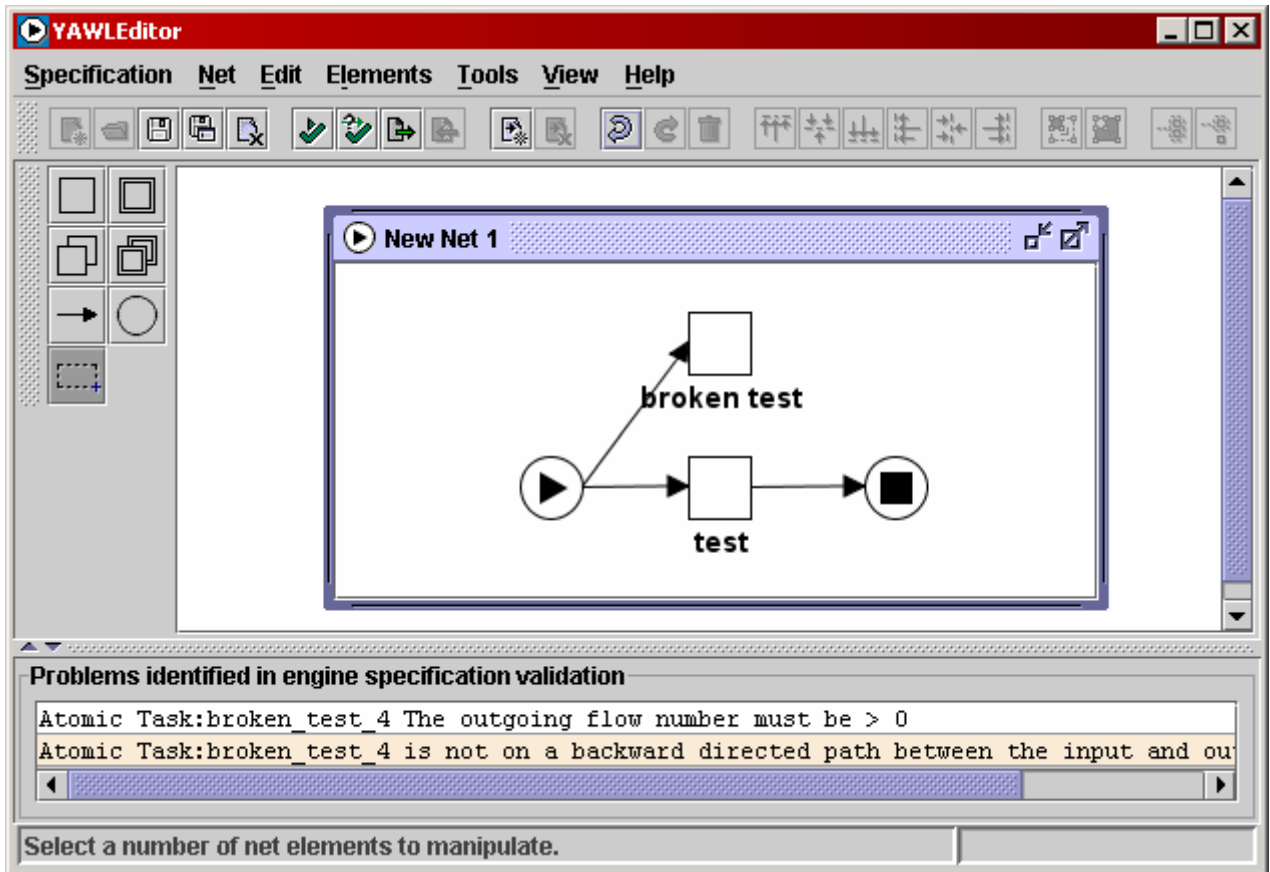
Fig. 39. An invalid specification
