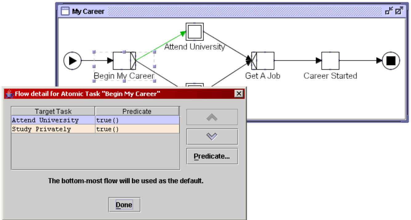
Fig. 34. Updating the Flow Detail
