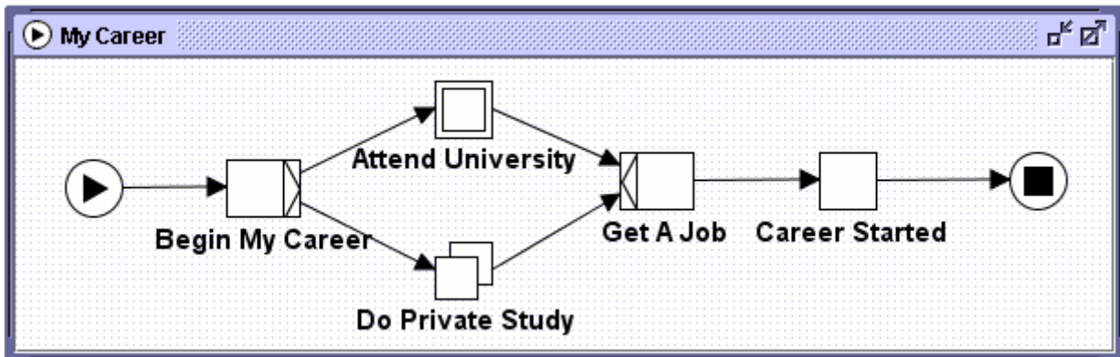
Fig. 10. Adding a Multiple Atomic Task
