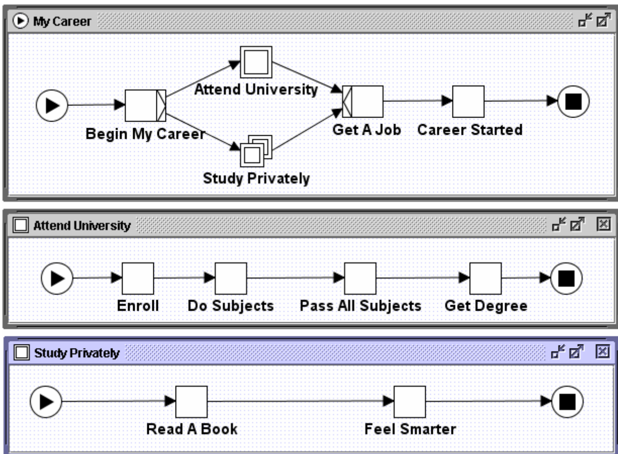
Fig. 12. "Privately Study" Multiple Composite Task and its Net
