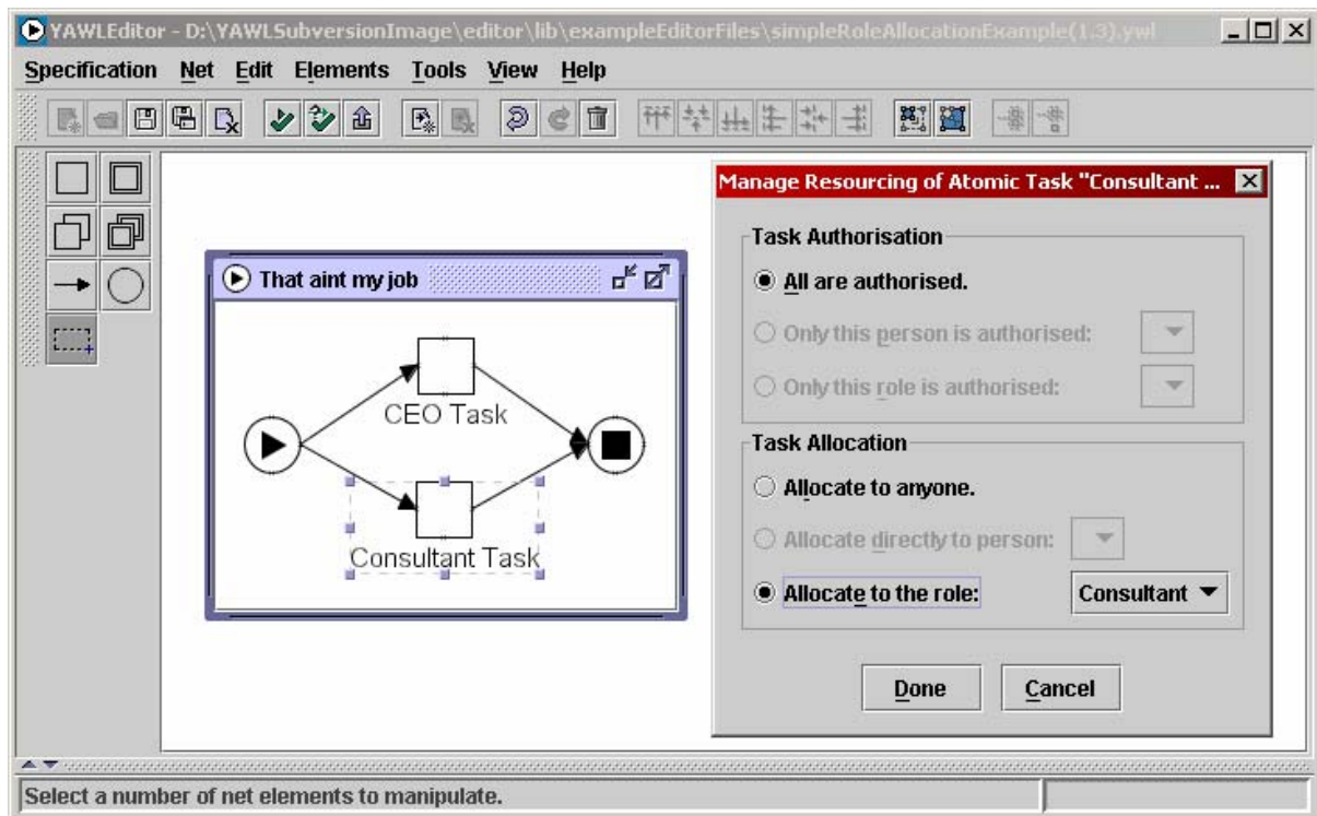
Fig. 47 Managing Resourcing of a task
