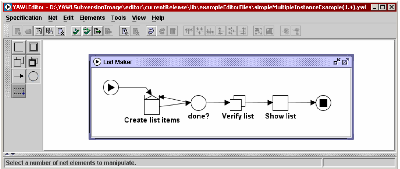
Fig. 42 - A simple specification showing how multiple instance tasks are done.
