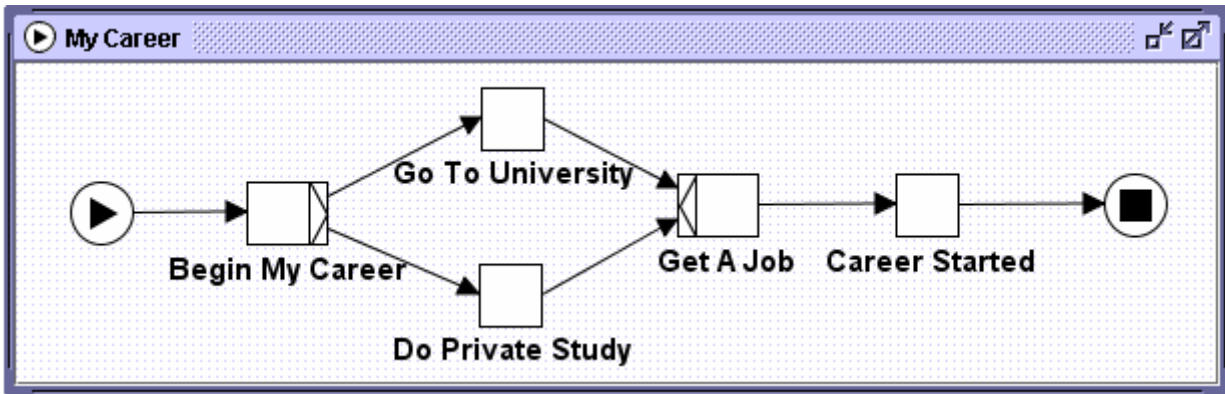
Fig. 8. XOR Split and Join
