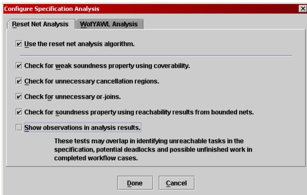
Fig. 40. Specification analysis functions
