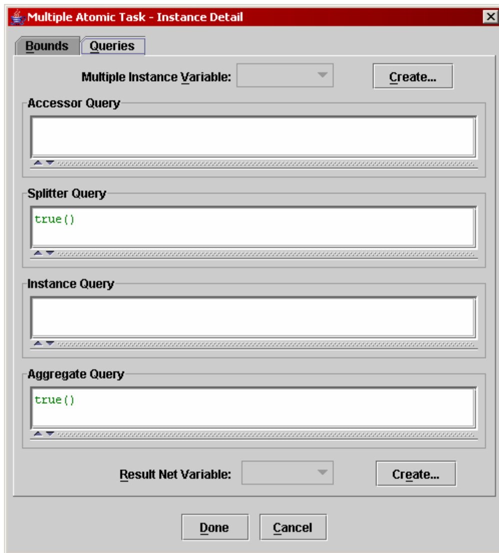
Fig. 37. Data Manipulation for Multiple Instance Tasks
