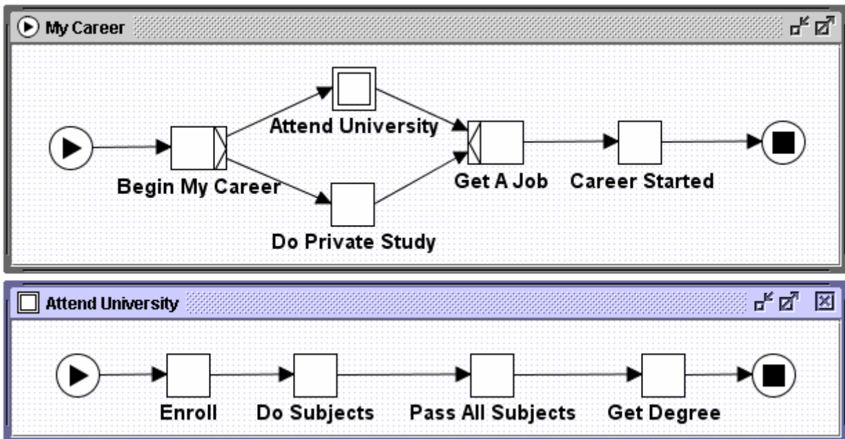
Fig. 9. "Attend University" Composite Task and its matching Net
