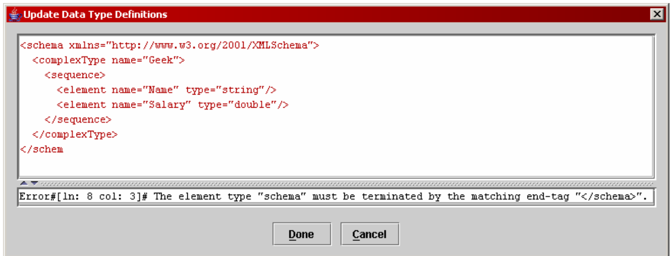
Fig. 22. When the "Geek" complex data type schema is invalid
