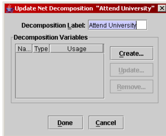
Fig. 24. Updating "Attend University" Net Variables
