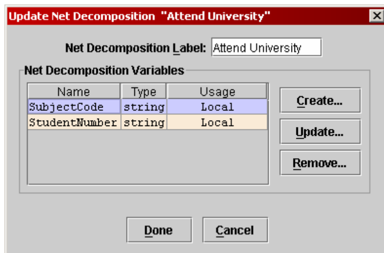
Fig. 26. Updated "Attend University" Net Variables
