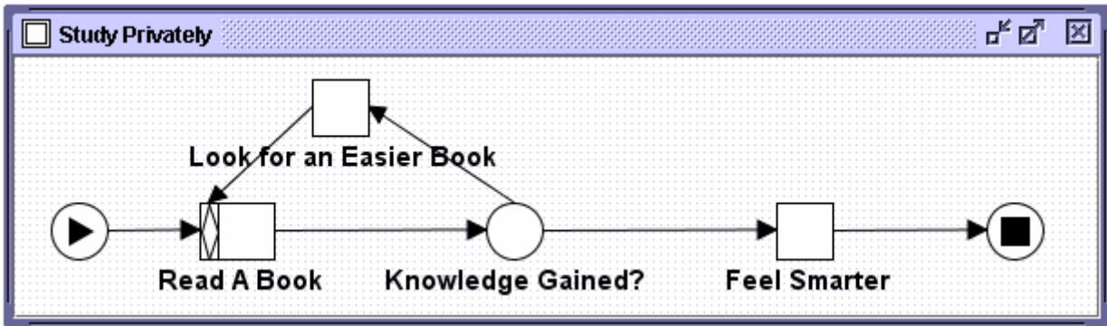
Fig. 13. Condition Loop for “Study Privately” Net
