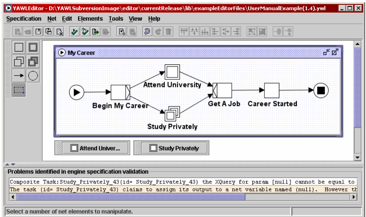
Fig. 14 - Validation with unfinished Multiple-Instance Tasks
