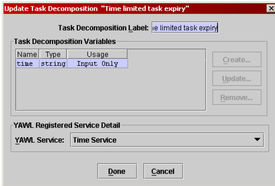
Fig. 46 - Assigning a registered YAWL service from a running engine
