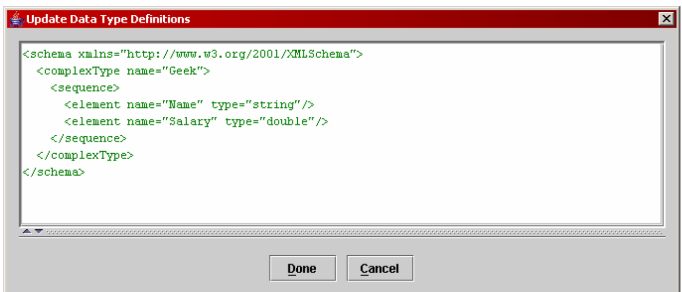
Fig. 21. Adding the "Geek" complex data type
