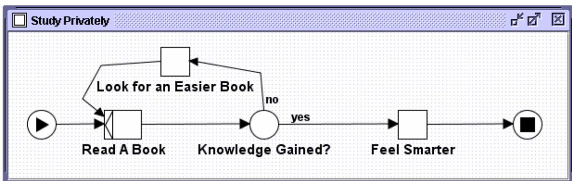
Fig. 17. Adding “knees” to a Flow Relation
