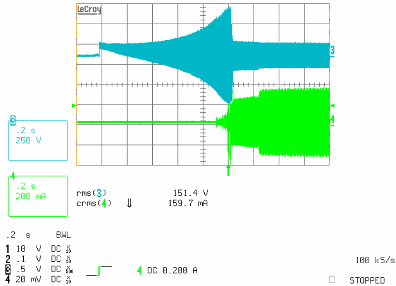
Figure 4.5: Lamp Voltage and Arc Current during preheat and ignition
