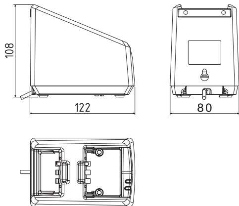
Desktop mounting, top view
