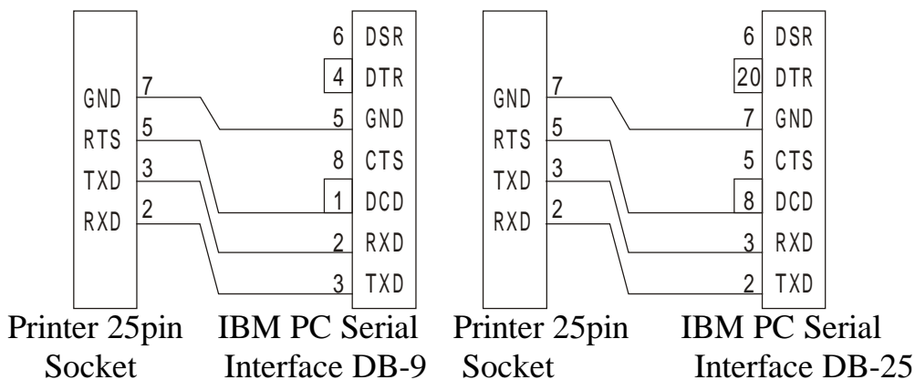
Fig.2-3 Connection between POS 76 II and IBM PC Serial Interface Sketch Map
