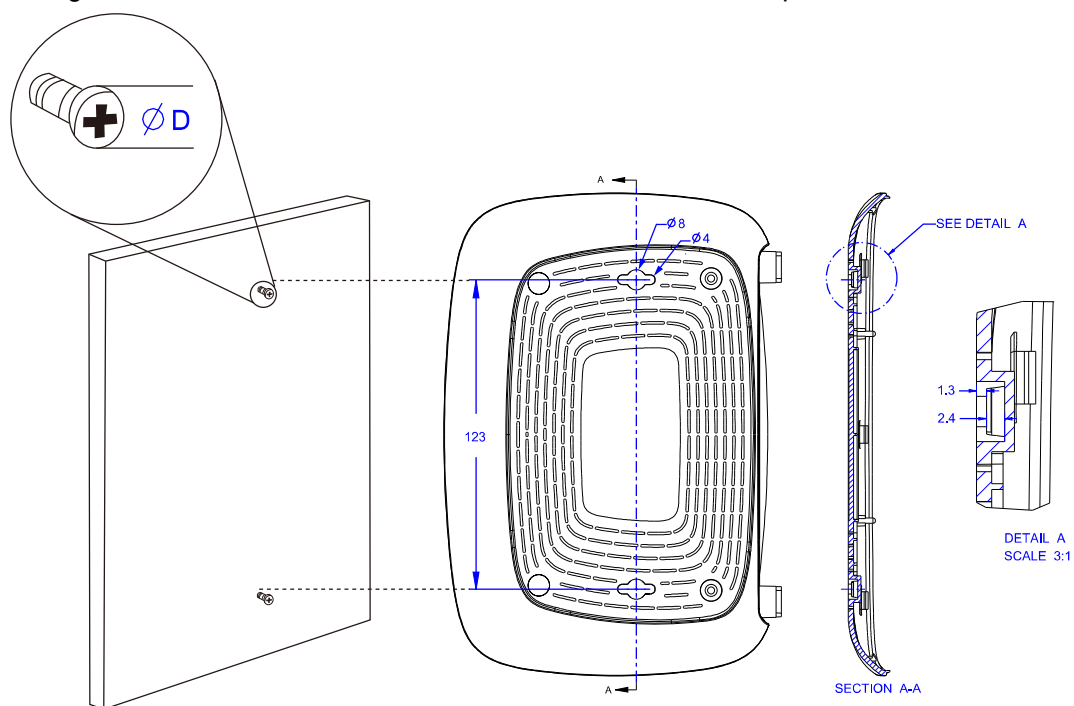
Figure 2-2 Wall-mount Install
