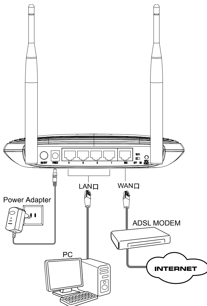
Figure 2-1 Hardware Installation of the TL-WR841ND 300Mbps Wireless N Router
