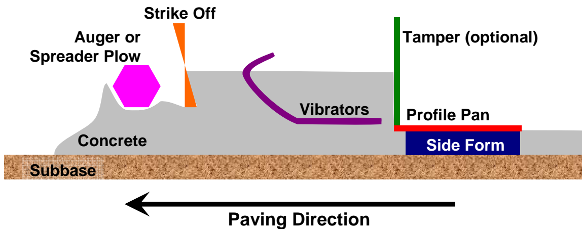
Figure 18. Typical components of a slipform paver.
