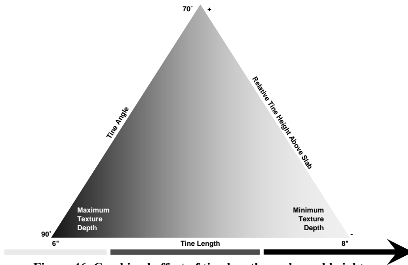
Figure 46. Combined effect of tine length, angle, and height.
