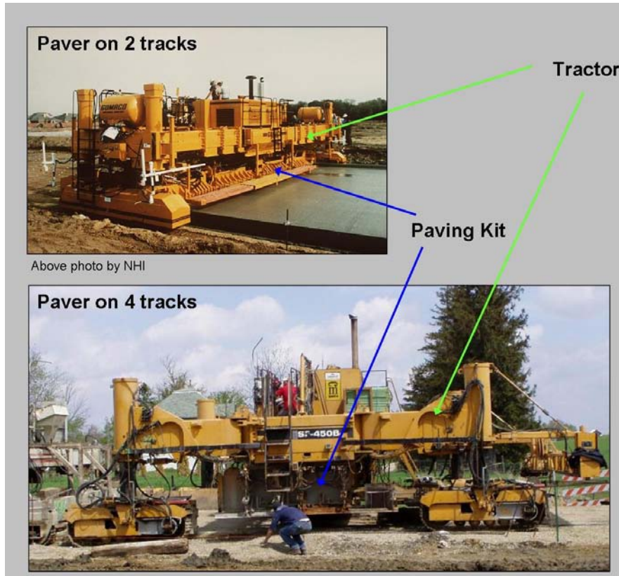
Figure 19. Two- and four-track pavers.
