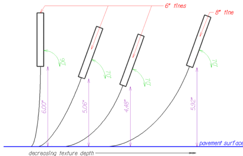
Figure 45. Relationship of texture depth to tine length, angle, and height.
