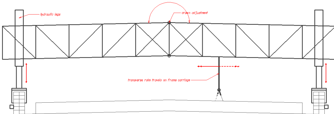
Figure 41. Schematic of transverse tining texture equipment.
