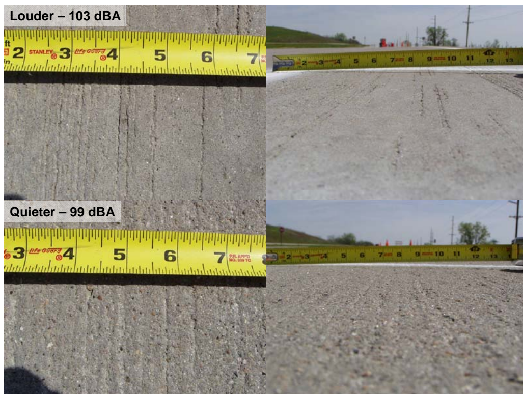
Figure 9. Variability of drag texture surface and its effect on OBSI noise level.
