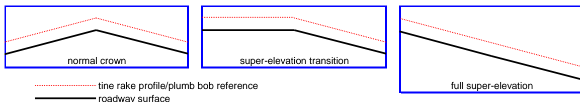
Figure 16. Pavement cross-slope adjustments.
