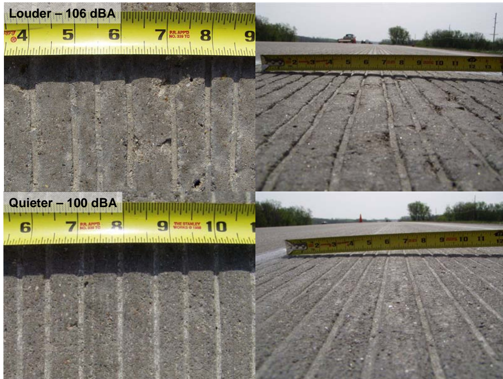
Figure 10. Variability of longitudinal tined surface and its effect on OBSI noise level.
