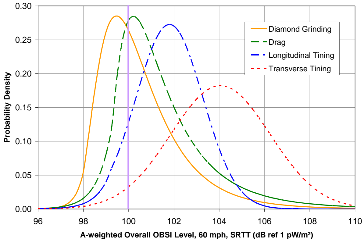
Figure 1. Normalized distributions of OBSI noise levels for conventional concrete pavement textures.
