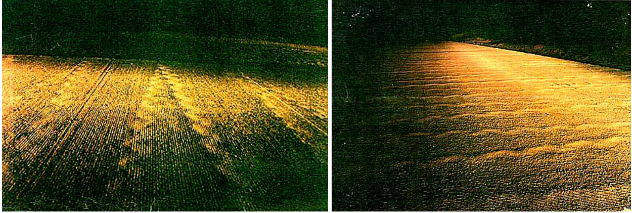
Figure 30. Unintended texture introduced by automatic longitudinal float.
