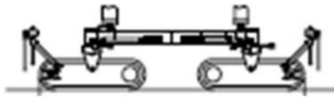
Figure 36. Side view schematic of the undercarriage of a four-track texture-cure machine.
