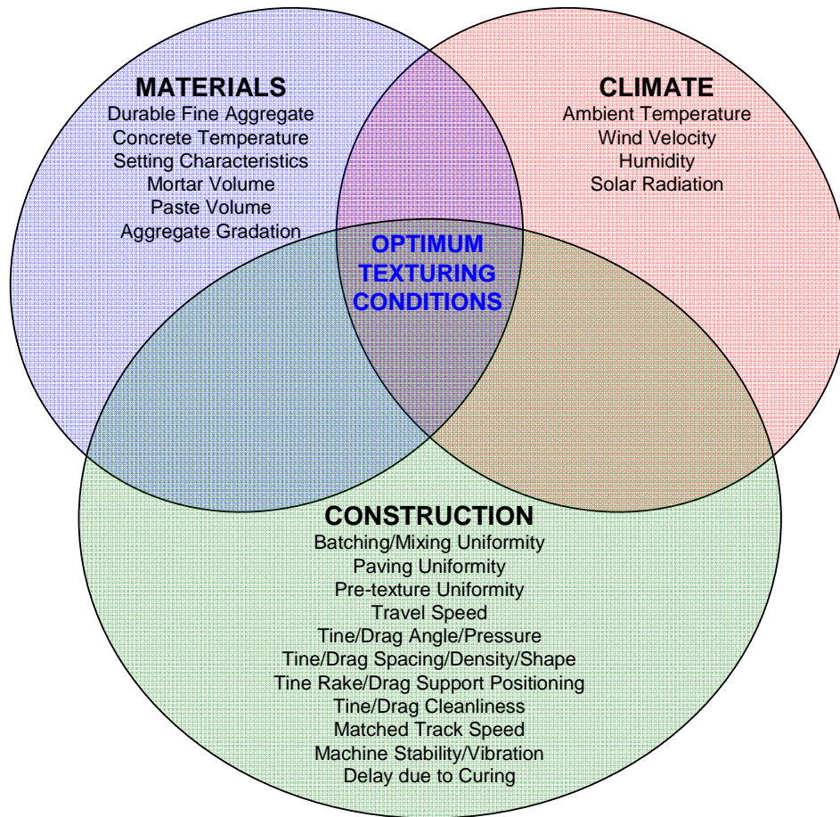
Figure 7. Variables affecting texture and the concept of an optimum texture window.
