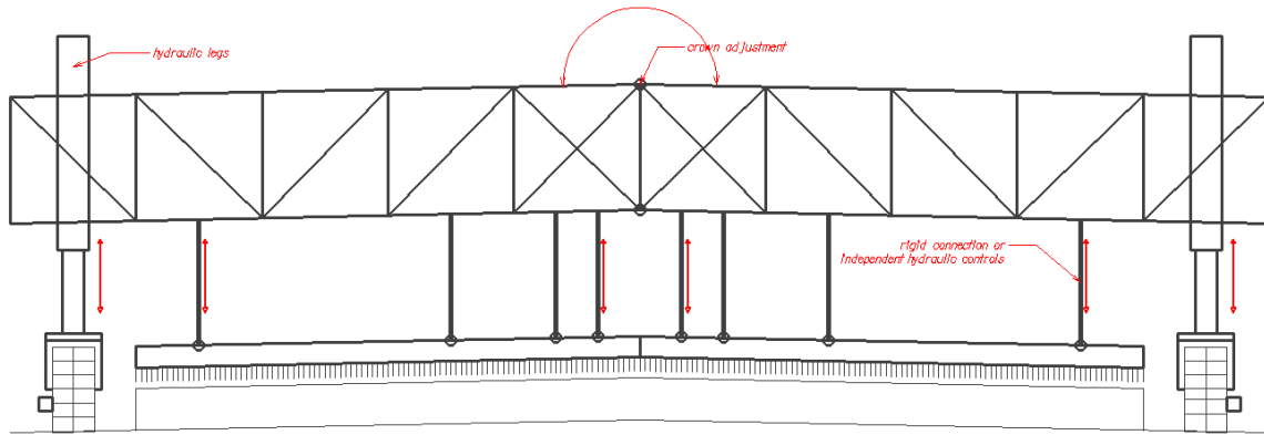
Figure 40. Schematic of longitudinal tining texture equipment.
