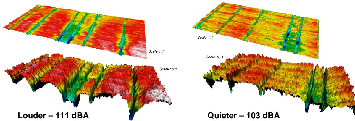
Figure 12. RoboTex scans of 100×200 mm samples showing variability of transverse tined surface and its effect on OBSI noise level.
