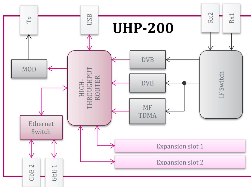
Figure 4 UHP-200 router structure
