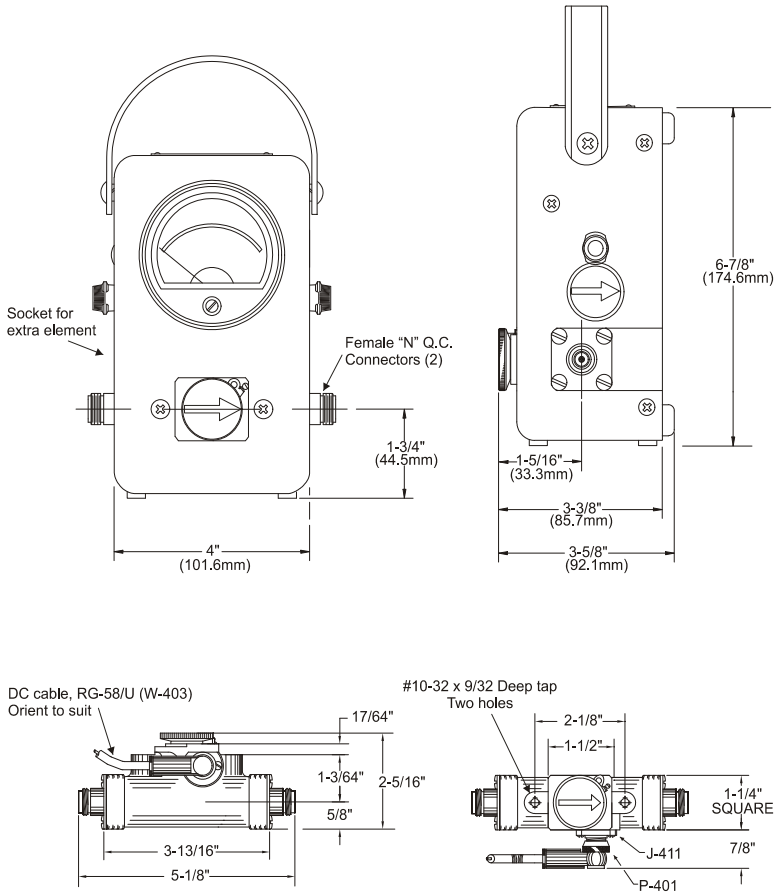
Figure 2 Bird 43 Thruline Wattmeter Outline Drawing
