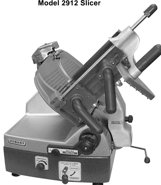
Model 2912 Slicer
