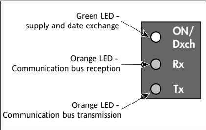
Figure 6-2 Interface status diagnostic LEDs
