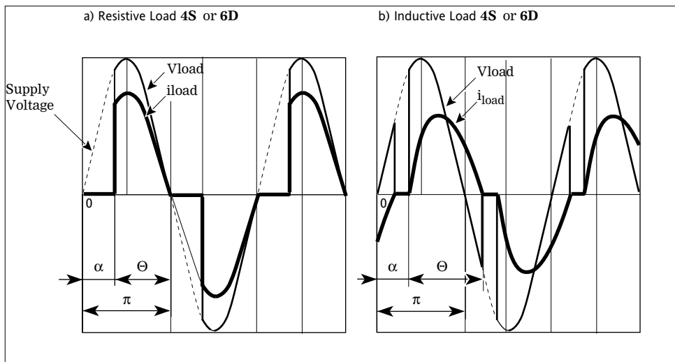
Figure 3-5 Voltage and current in one phase of a three-phase load (code 4S or 6D) in 'Phase angle' mode a) - resistive load; b) - inductive load.
