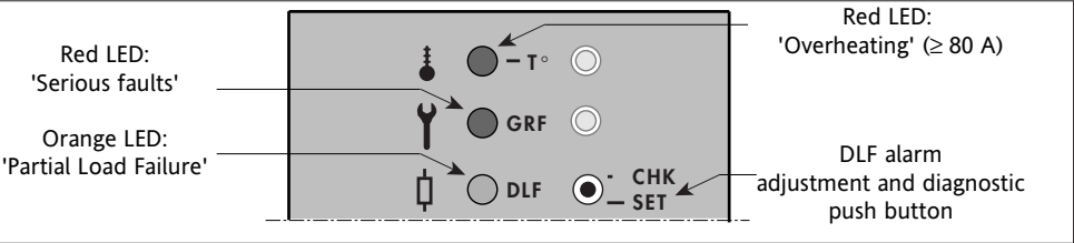
Figure 5-1 Layout of front panel LEDs with 'GRF' and/or 'DLF' option
