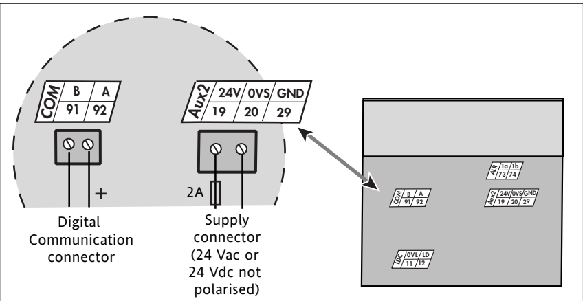
Figure 2-16 Power supply connection diagram
