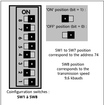
Figure 6-1 Example : Switch positions.
