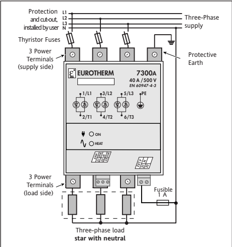
Figure 2-8 Connecting a three-phase load using star with neutral configuration (4S) Note : Connection to EXT terminal only with DLF or VICL options.
