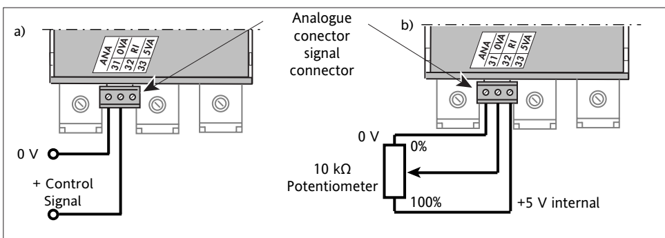
Figure 2-11 Control signal connection (self-powered unit, base version)
