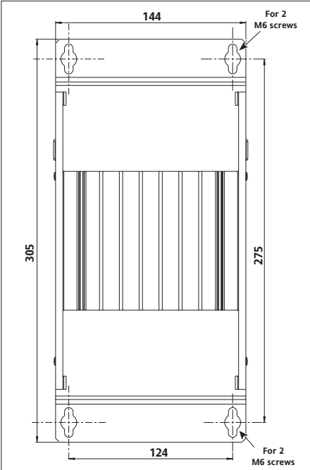
Figure 2-3 Bulkhead mounting - 63 A to 100 A units
