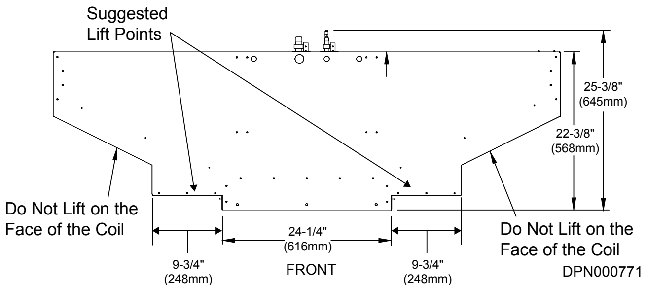
Figure 8 Liebert XDO lift points
