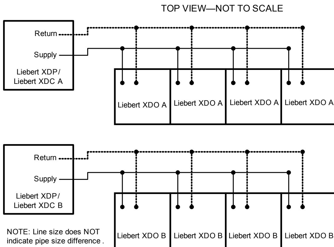
Figure 18 Typical Liebert XDO piping—non-interlaced connection
