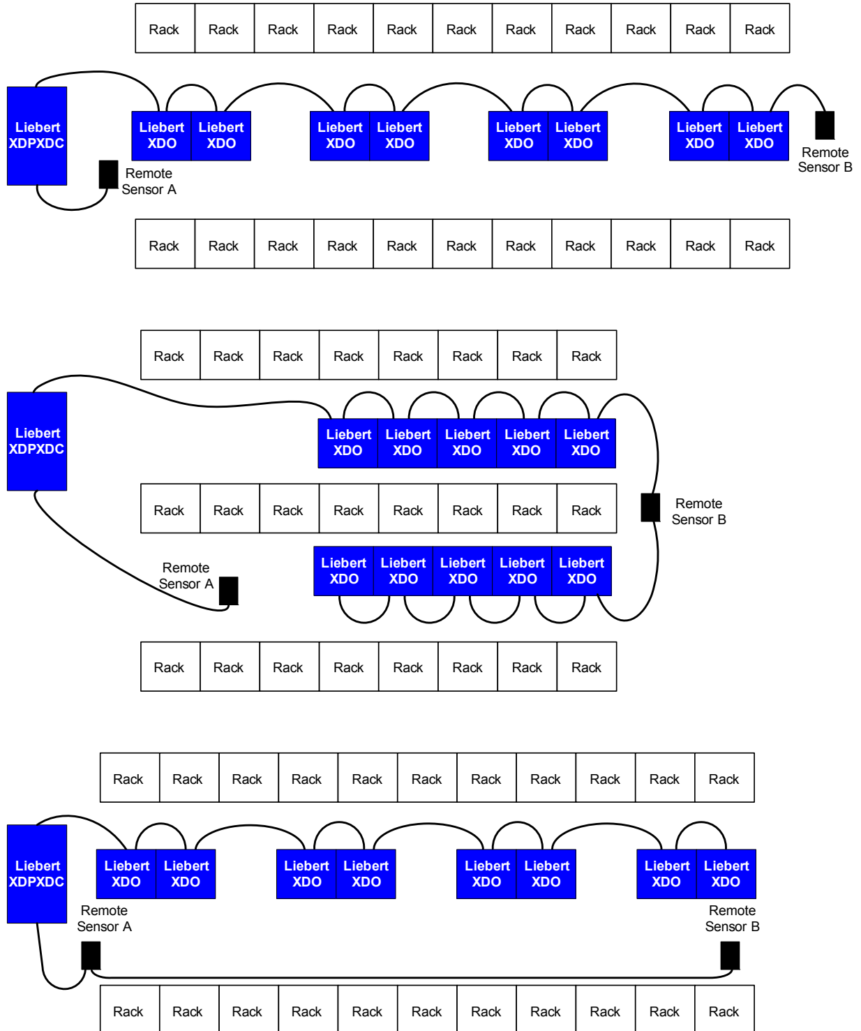
Figure 45 Modules on a single chain
