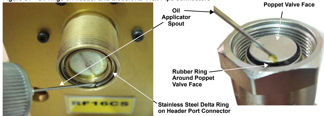
Figure 31 Oil rings on header and Liebert XD Flex Pipe connectors
