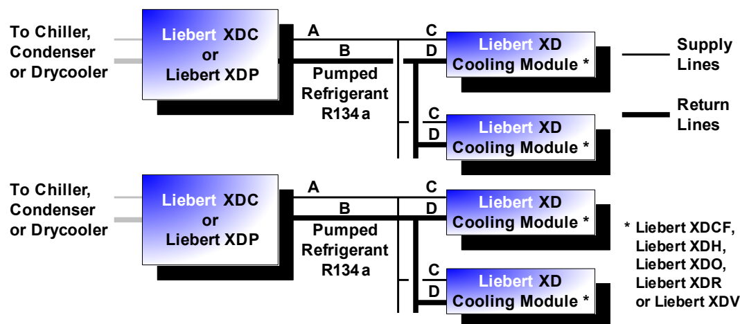
Figure 22 Generic piping layout
