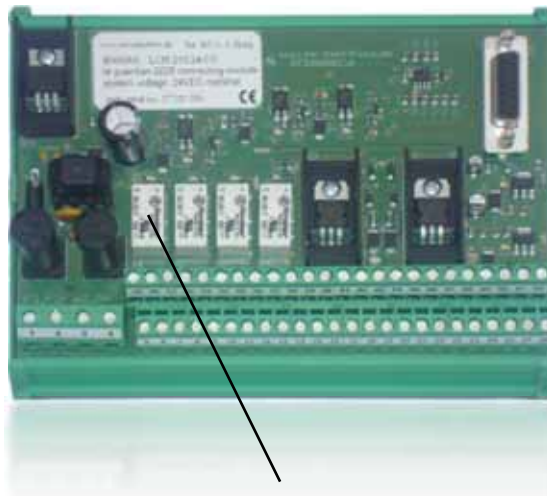
system fail relay K1 with control LED 1
