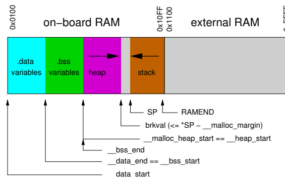
Figure 6: RAM map of a device with internal RAM
