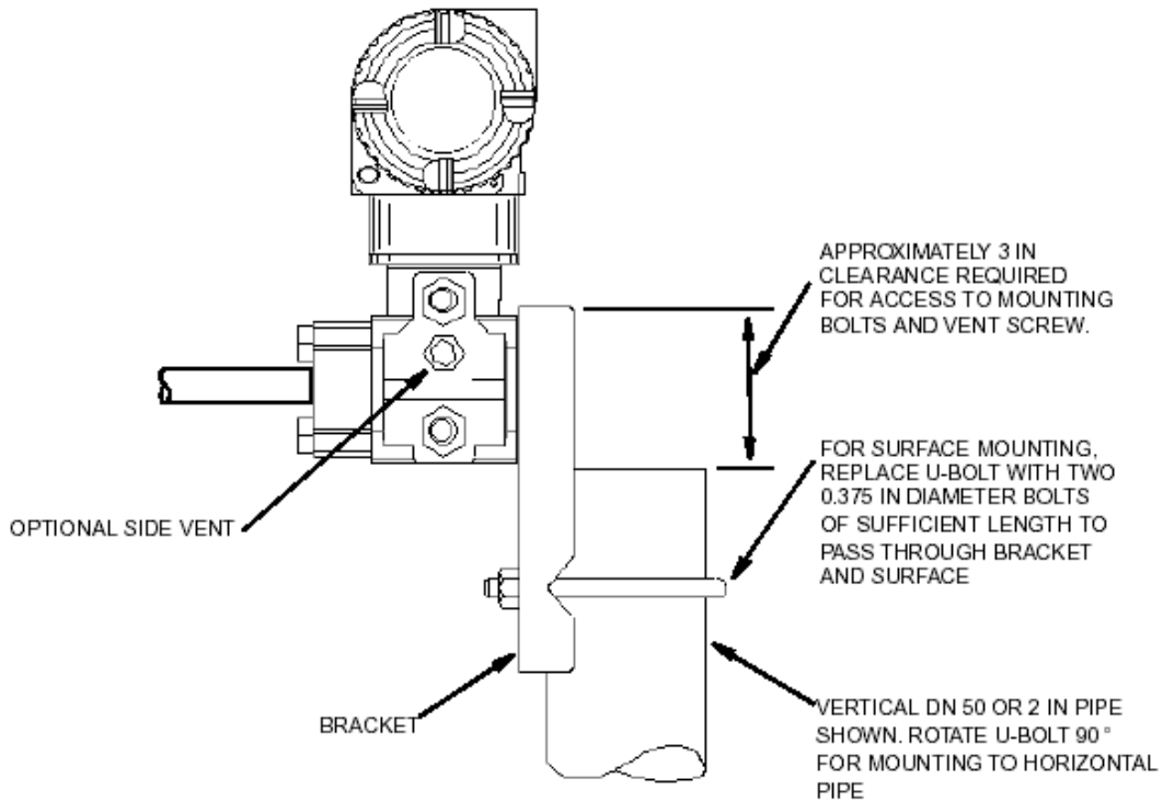
Figure 2: Mounting the SCADASense 4203 DR Series to a Pipe or Surface
