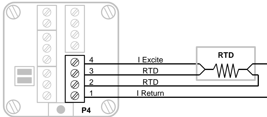
Figure 12: Transmitter 4-Wire RTD Wiring
