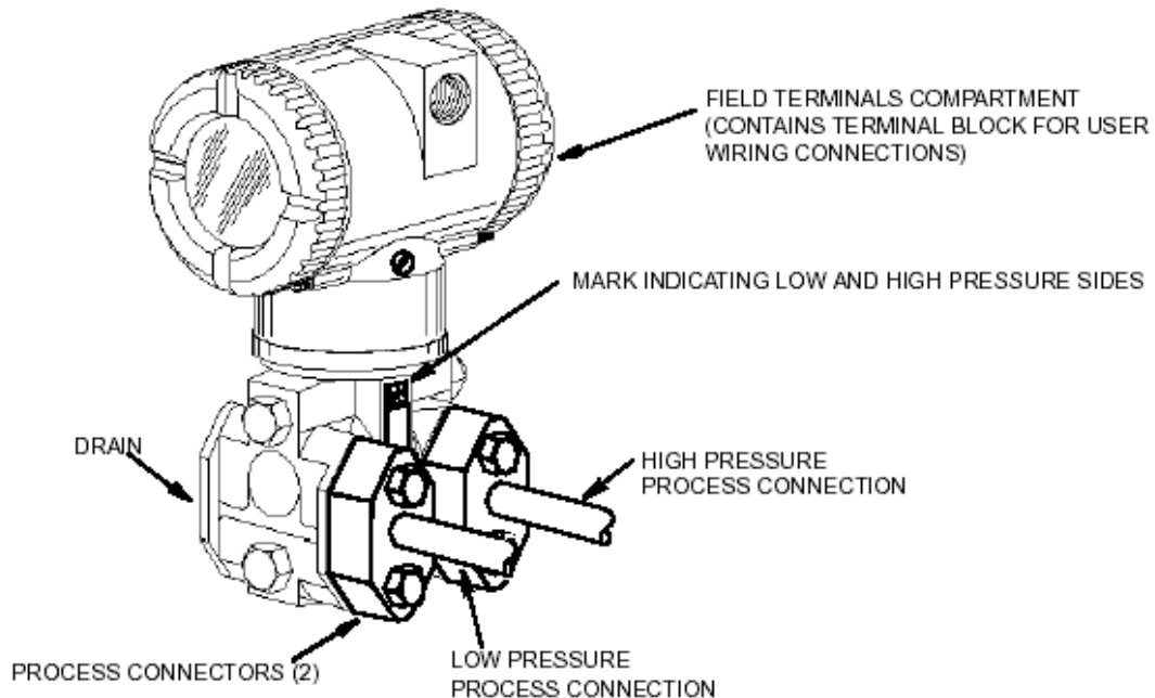
Figure 1: Process-Mounted GFC
