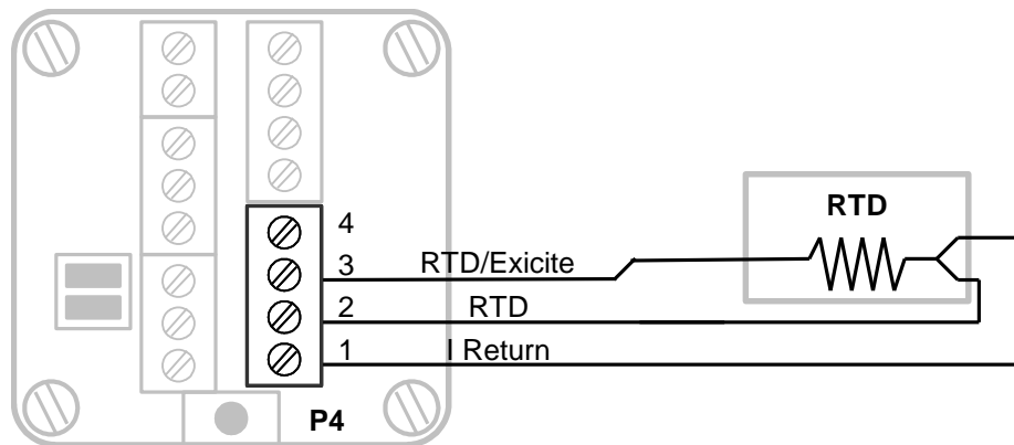
Figure 13: Transmitter 3-Wire RTD Wiring
