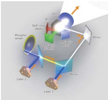
Light source and optical light path image
