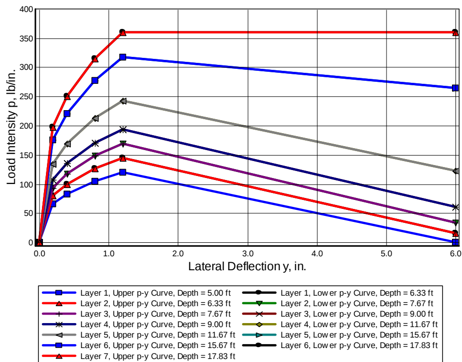
Figure 5-28 User-input p - y Curves for Example 7 (Lower curve for Layer 7 not shown)
