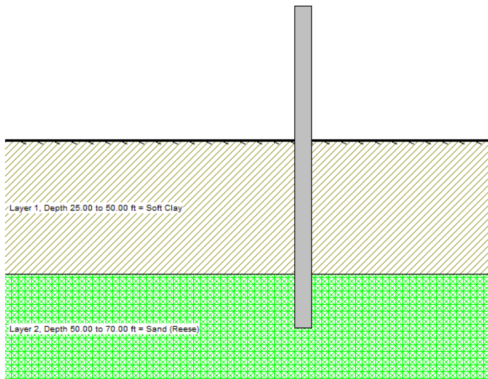
Figure 5-62 Pile and Soil Profile for Verification of P-Delta Effect
