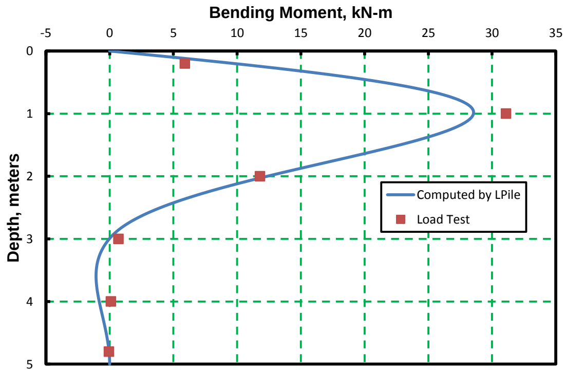
Figure 5-31 Comparison between Measured and Computed Bending Moment versus Depth for the 5-m Pile of Example 8
