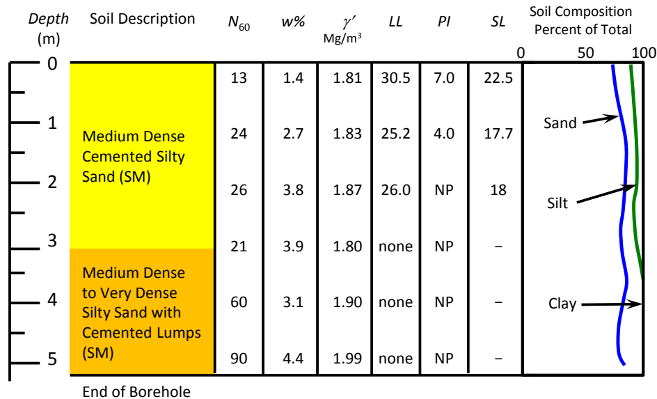
Figure 5-29 Soil details for Example 8
