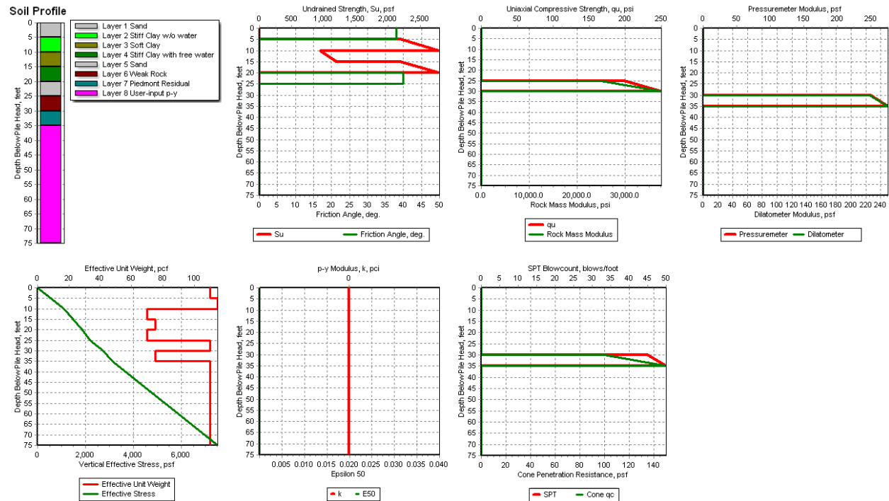
Figure 4-3 Example of Summary Graphs of Soil Properties
