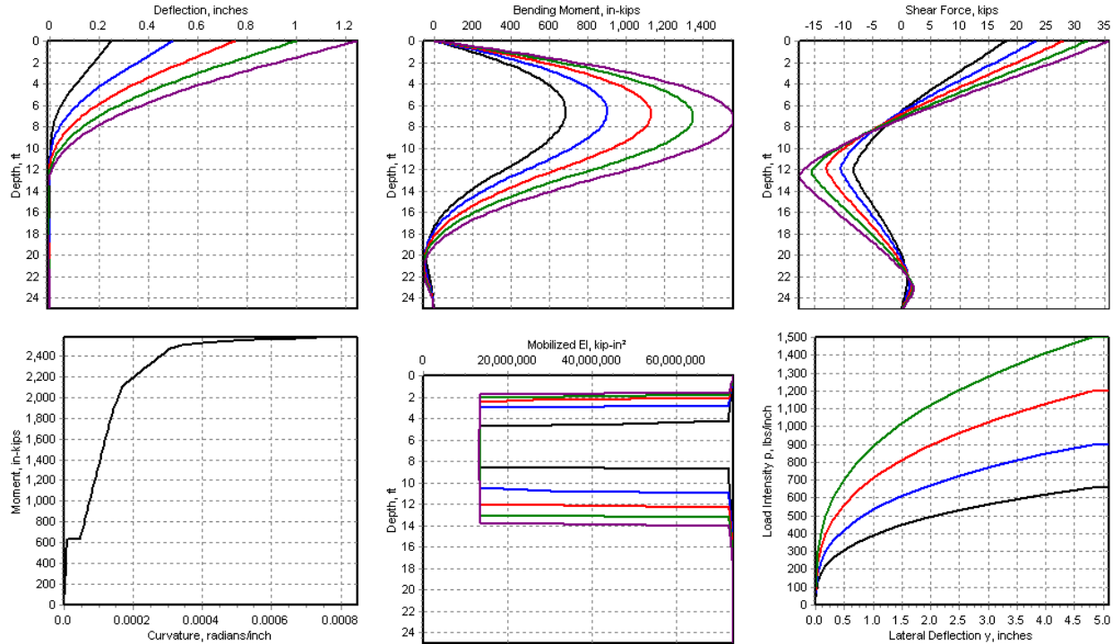
Figure 5-36 Summary Plots of Results for Example 10
