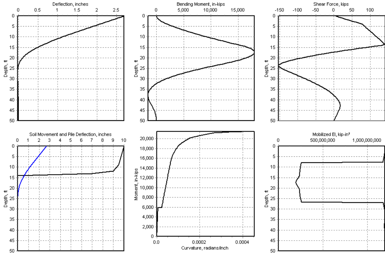
Figure 5-61 Results of Analysis for Example 24
