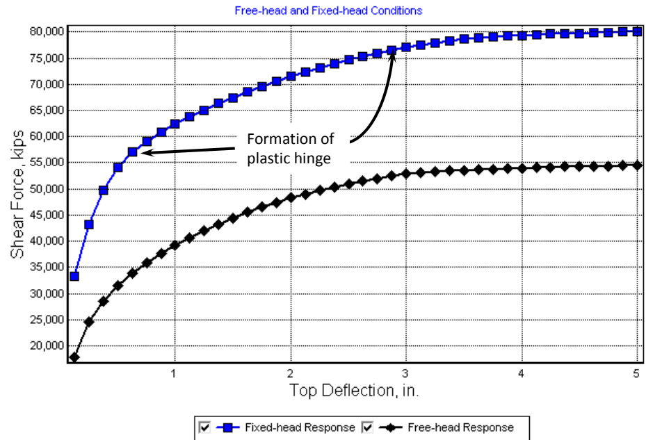
Figure 3-43 Pile-head Shear Force versus Displacement from Pushover Analysis
