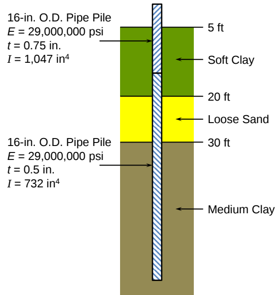
Figure 5-27 Pile and soil details for Example 7
