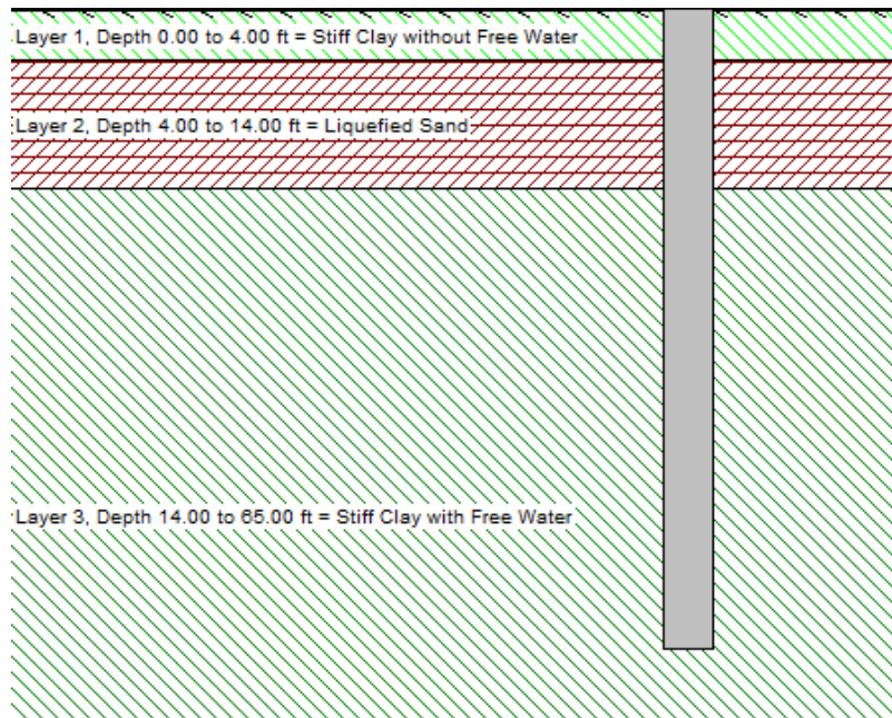
Figure 5-58 Pile and Soil Profile for Example 24
