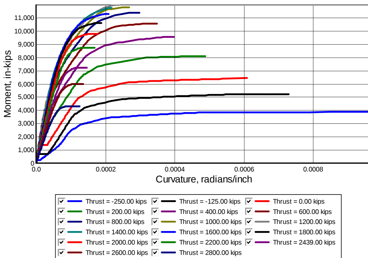
Figure 5-22 Moment versus Curvature for Example 5
