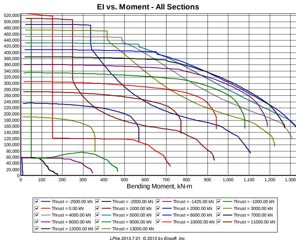
Figure 5-10 Bending Stiffness versus Bending Moment for Example 2a.
