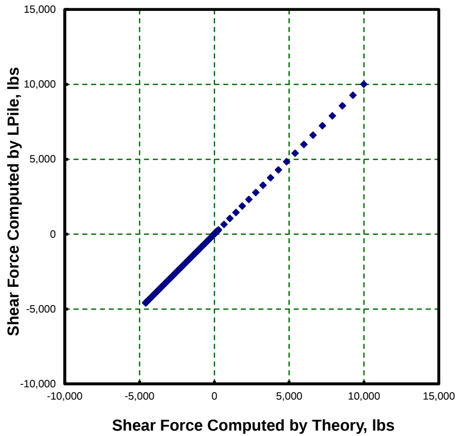
Figure 6-7 Verification of Shear Forces
