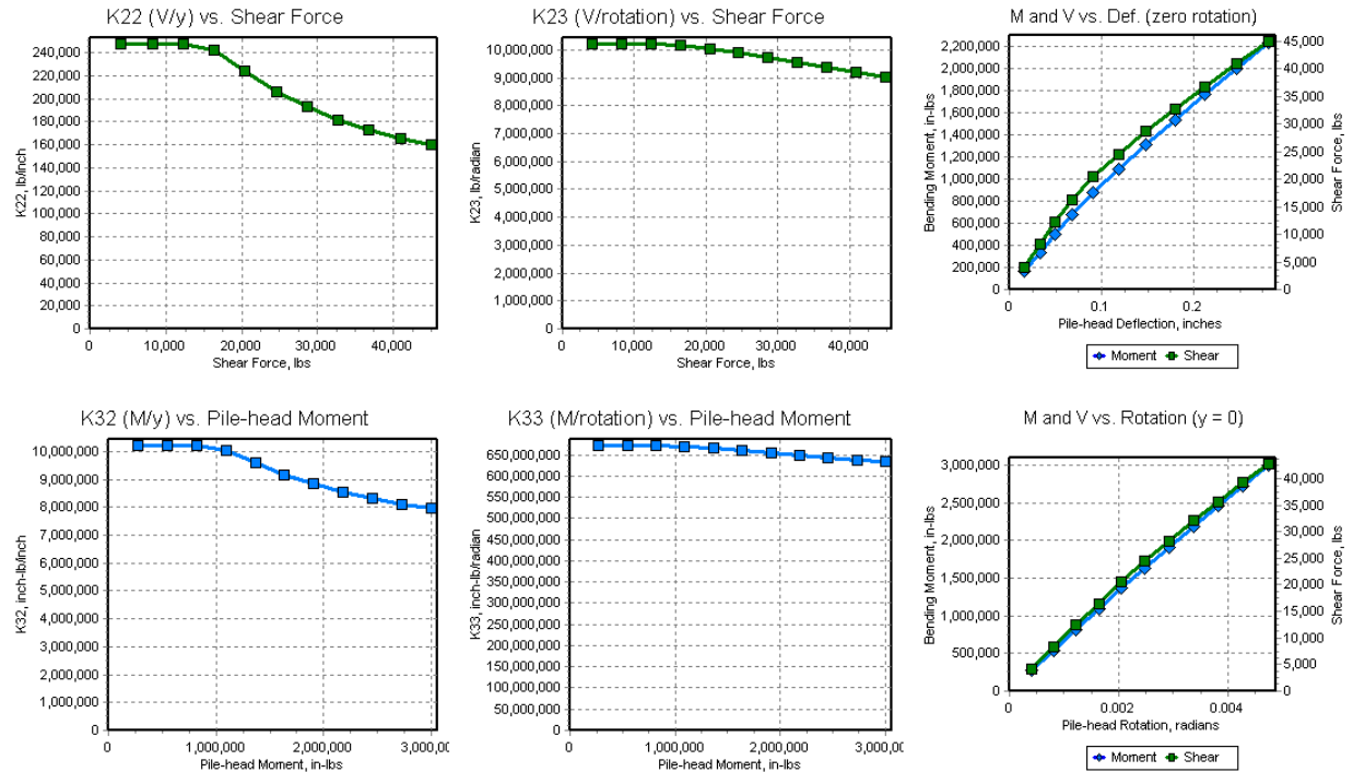
Figure 5-26 Stiffness Matrix Components versus Force and Moment, Example 6
