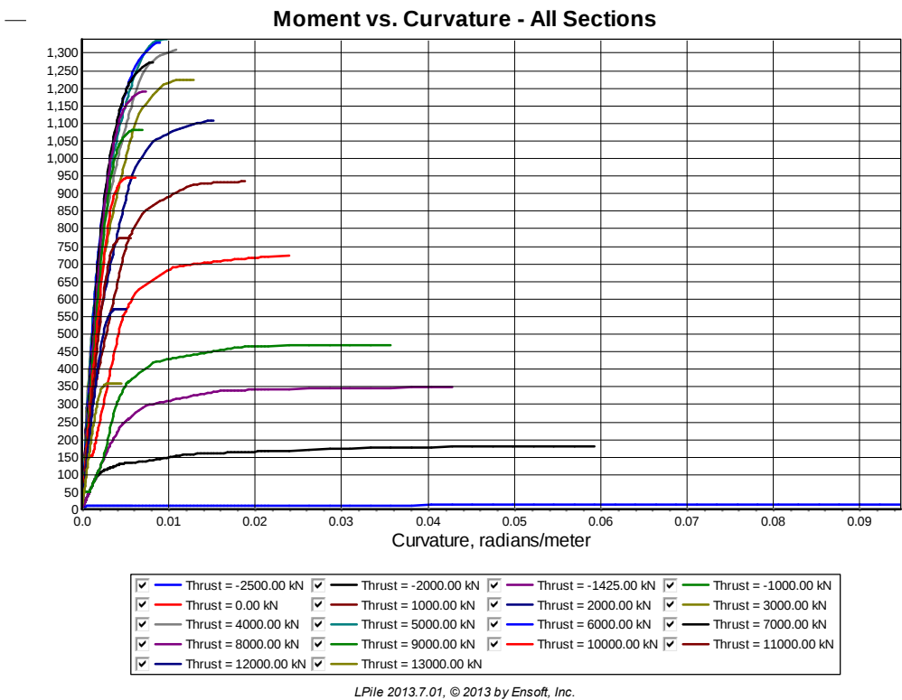
Figure 5-9 Moment-Curvature Diagram for Example 2a.
