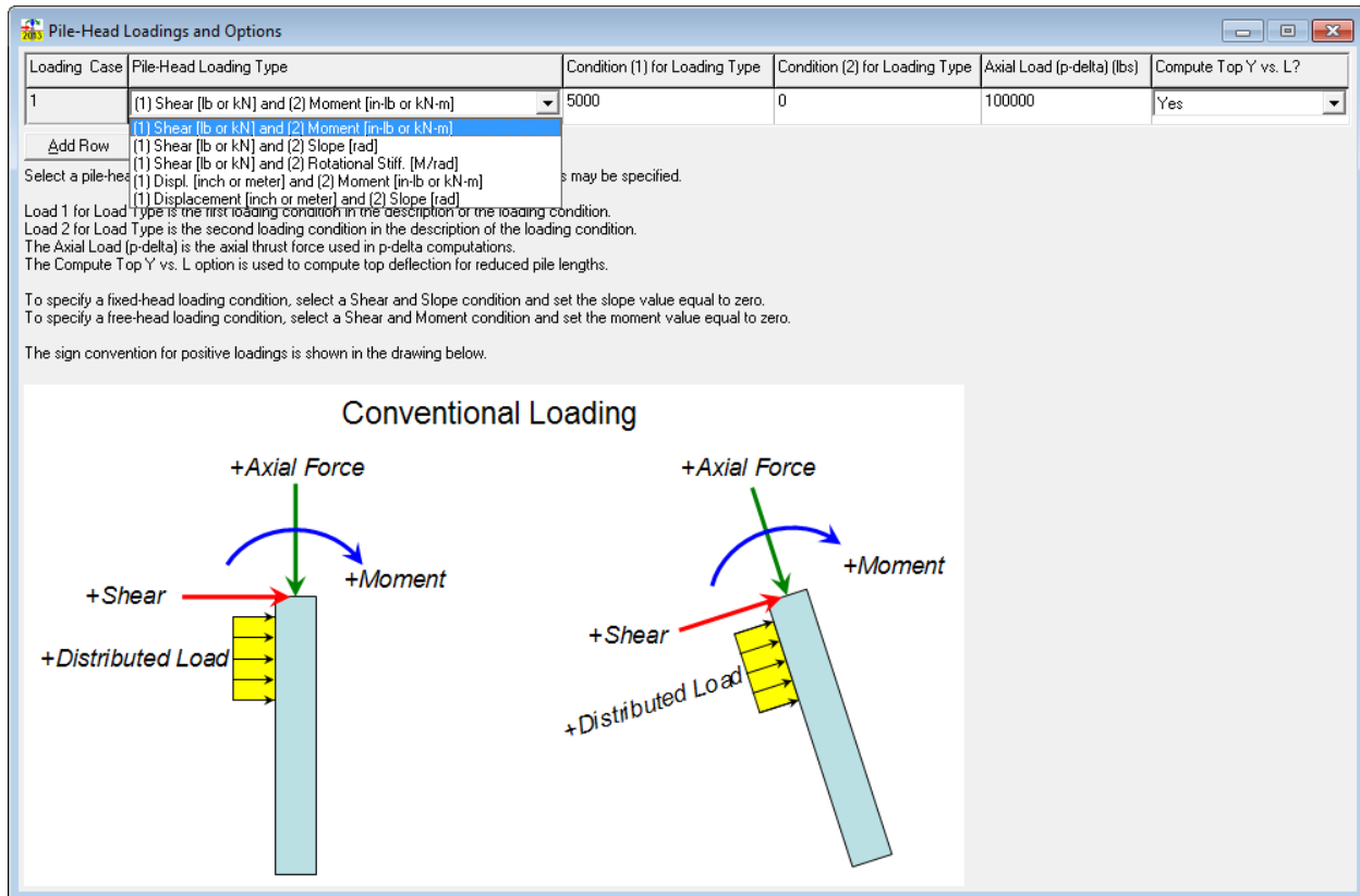
Figure 3-35 Dialog for Definition of Conventional Pile-head Loading
