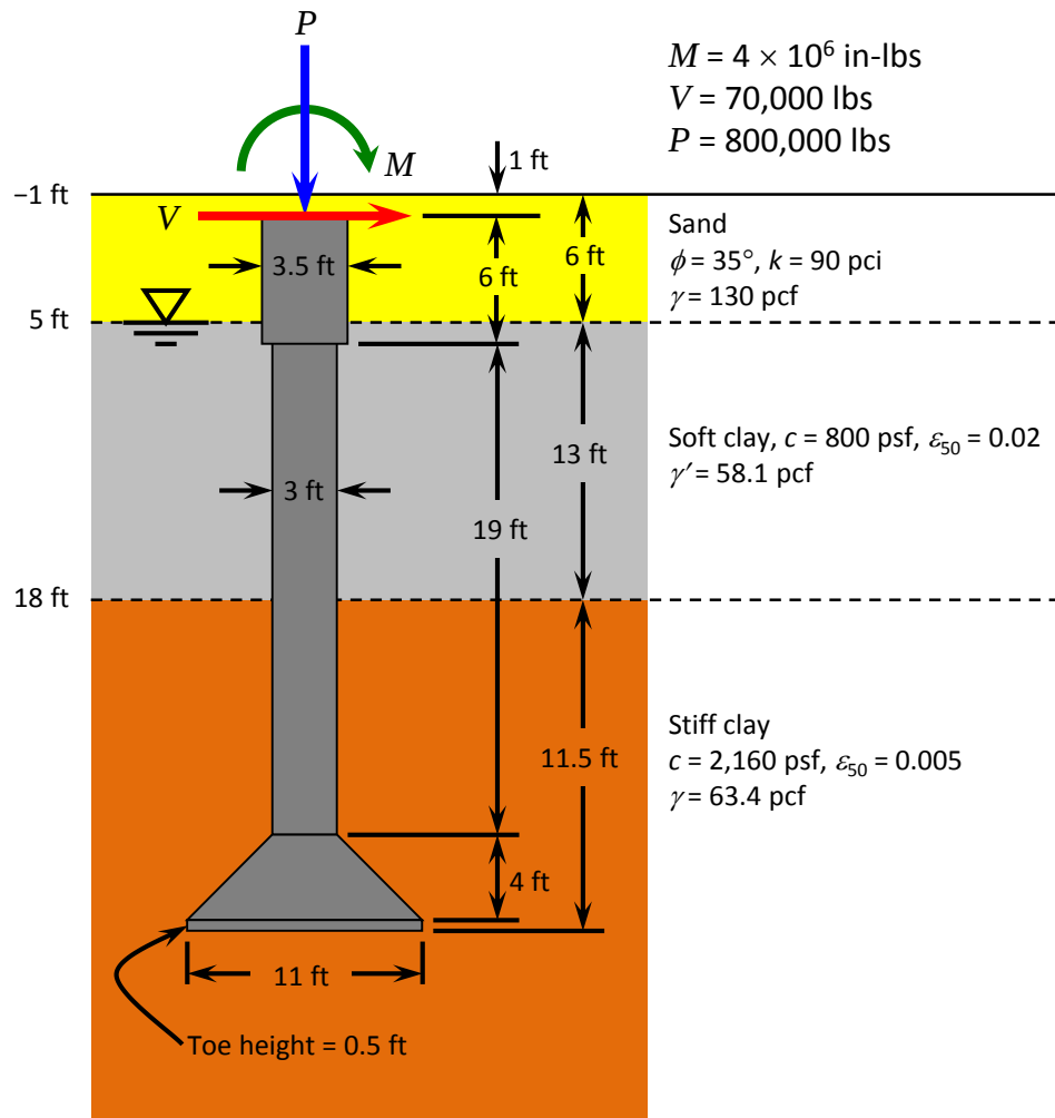
Figure 5-32 Shaft and Soil Details for Example 9
