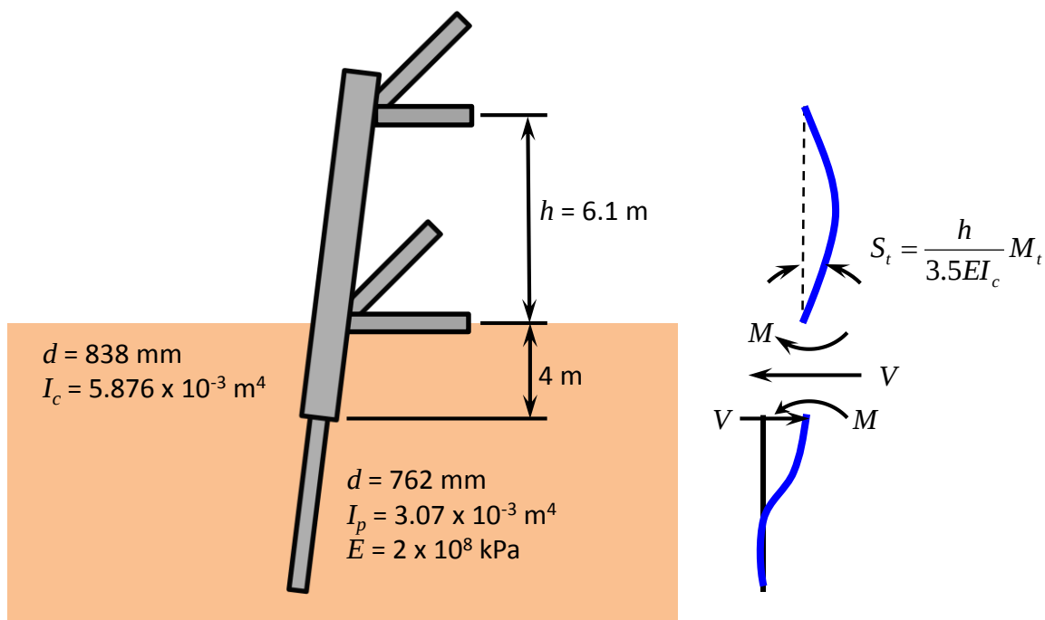
Figure 5-16 Superstructure and Pile Details, Example 3
