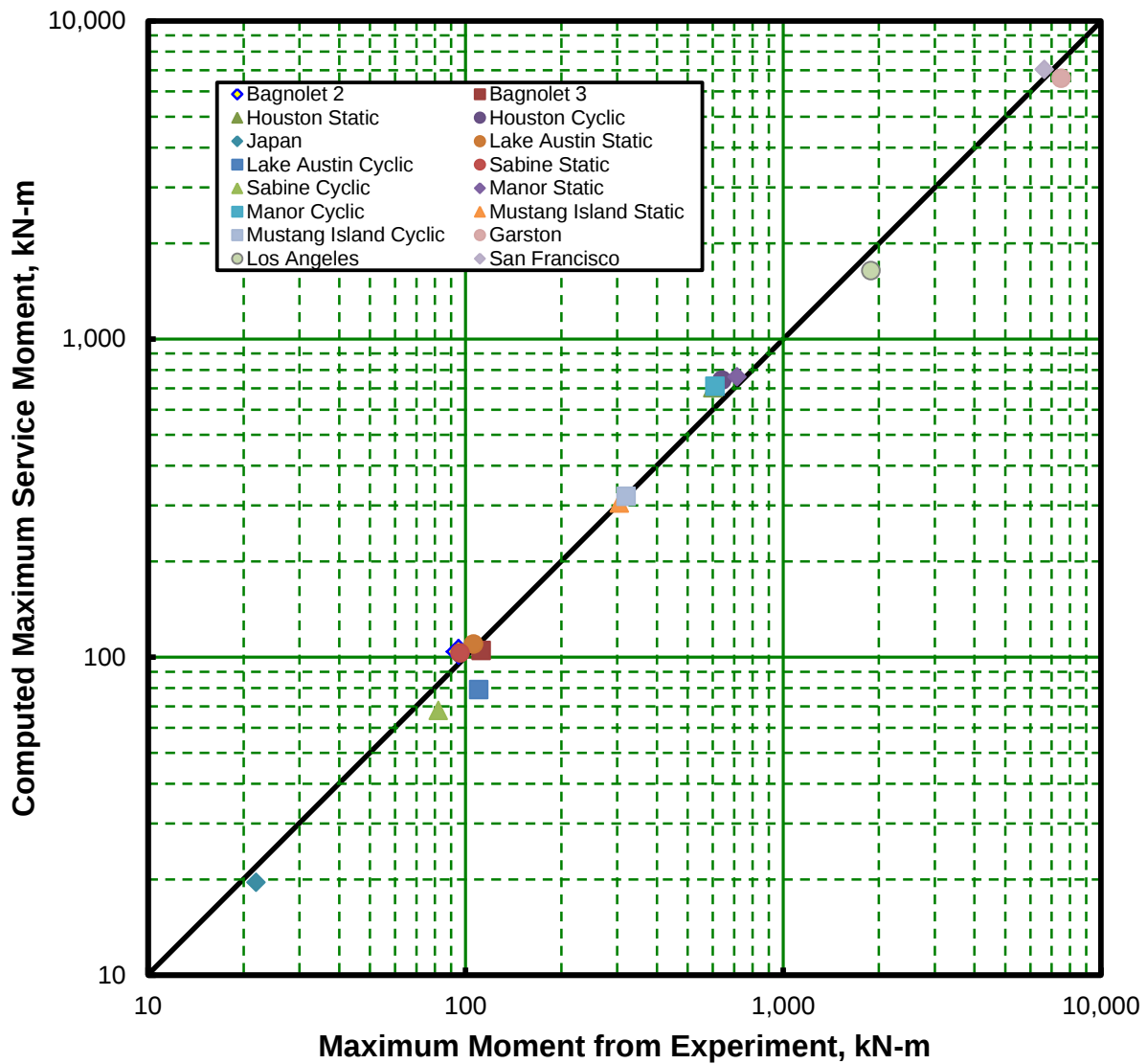
Figure 6-1 Comparison of Maximum Bending Moments from Computations and from Experimental Case Studies
