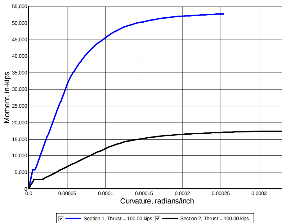
Figure 5-50 Moment versus Curvature for Dual Section Drilled Shaft with Permanent Casing and Core of Example 19
