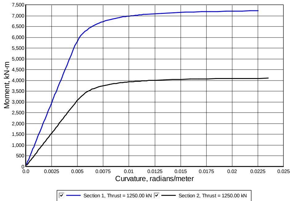
Figure 5-17 Moment versus Curvature, Example 3
