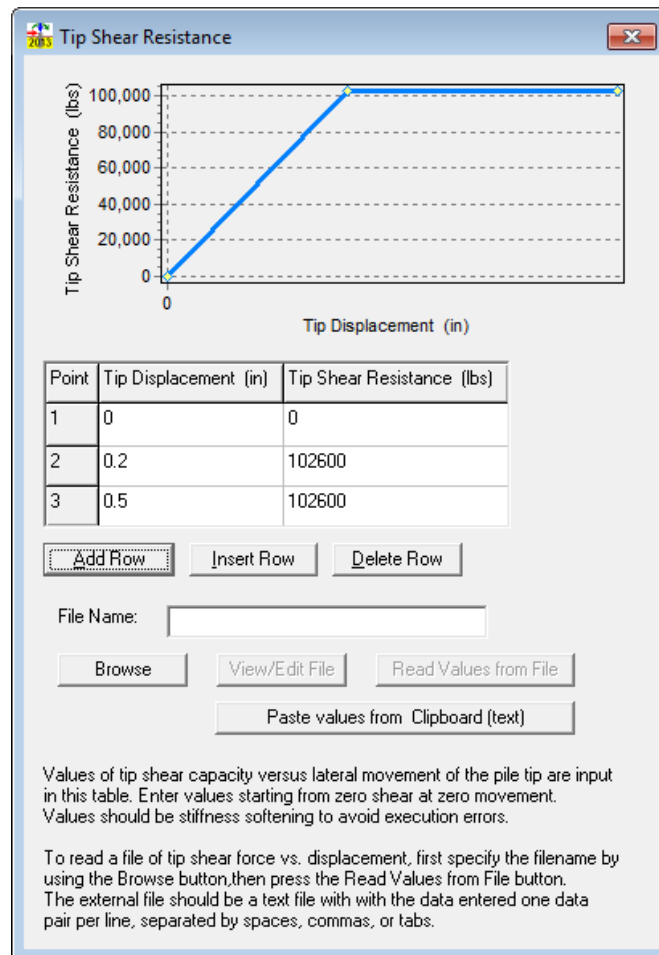
Figure 3-31 Dialog for Tip Shear Resistance versus Lateral Tip Displacement
