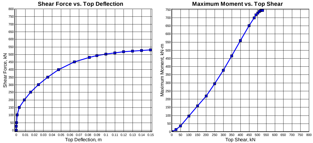
Figure 5-11 Shear Force versus Top Deflection and Maximum Bending Moment versus Top Shear Load for Free-head Conditions in Example 2b.
