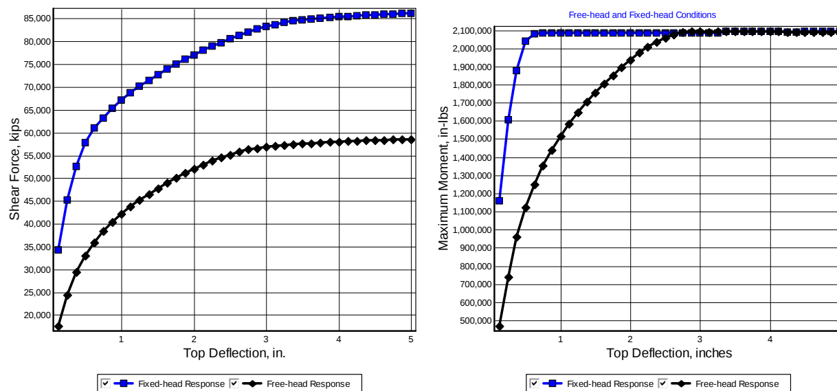
Figure 5-46 Results of Pushover Analysis of Prestressed Concrete Pile of Example 14
