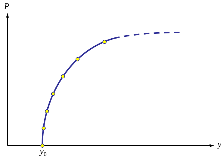
Figure 3-46 Typical Results for a Pile Buckling Analysis
