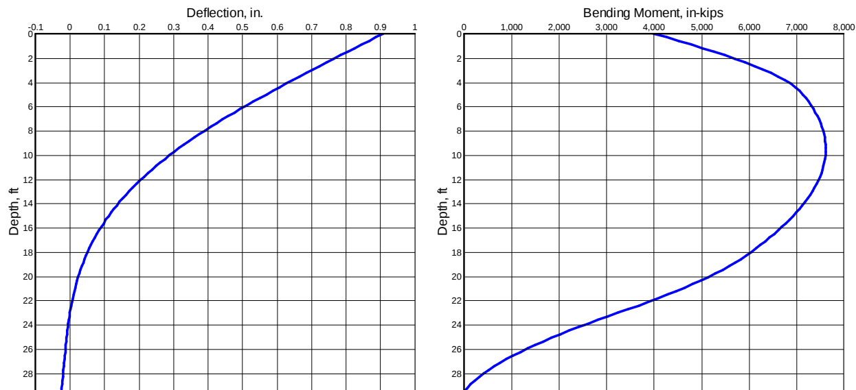
Figure 5-34 Lateral Deflection and Bending Moment versus Depth, Example 9
