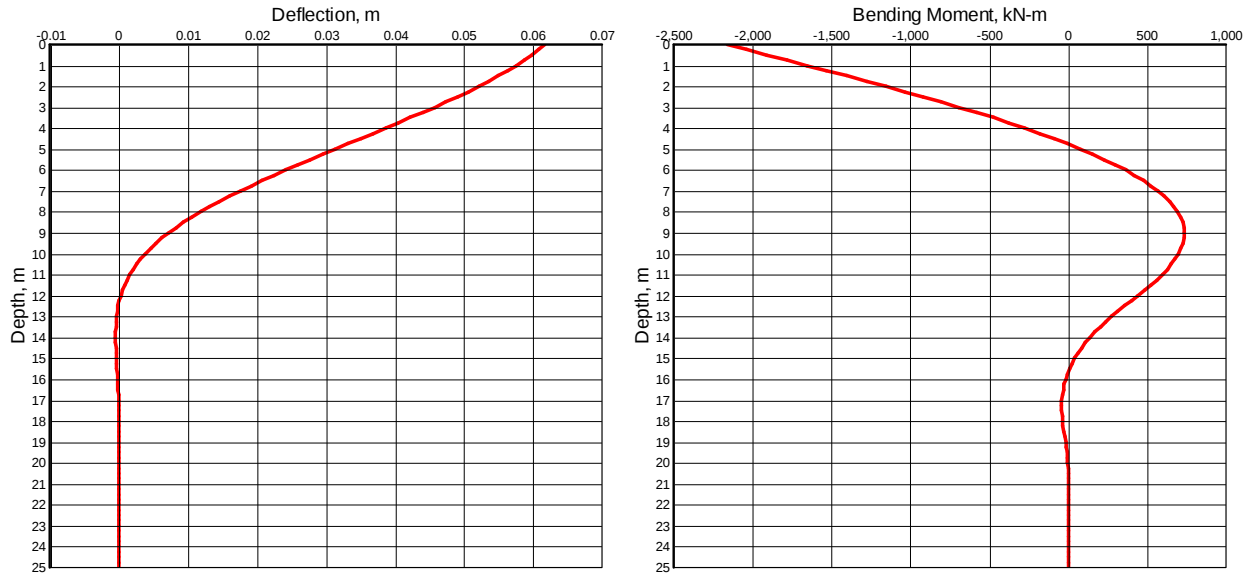
Figure 5-19 Pile Deflection and Bending Moment versus Depth for V_{top} = 500 kN, Example 3
