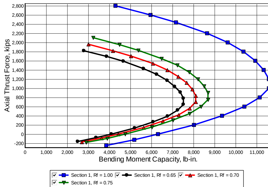
Figure 5-24 Factored Interaction Diagram of Reinforced-concrete Pile, Example 5
