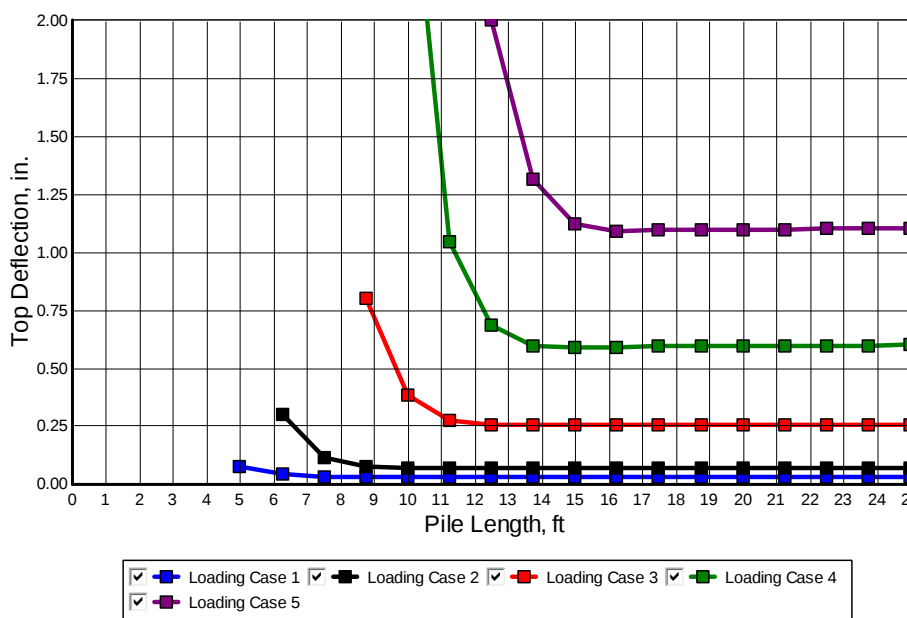
Figure 5-43 Curves of Pile Top Deflection versus Pile Length for Example 13
