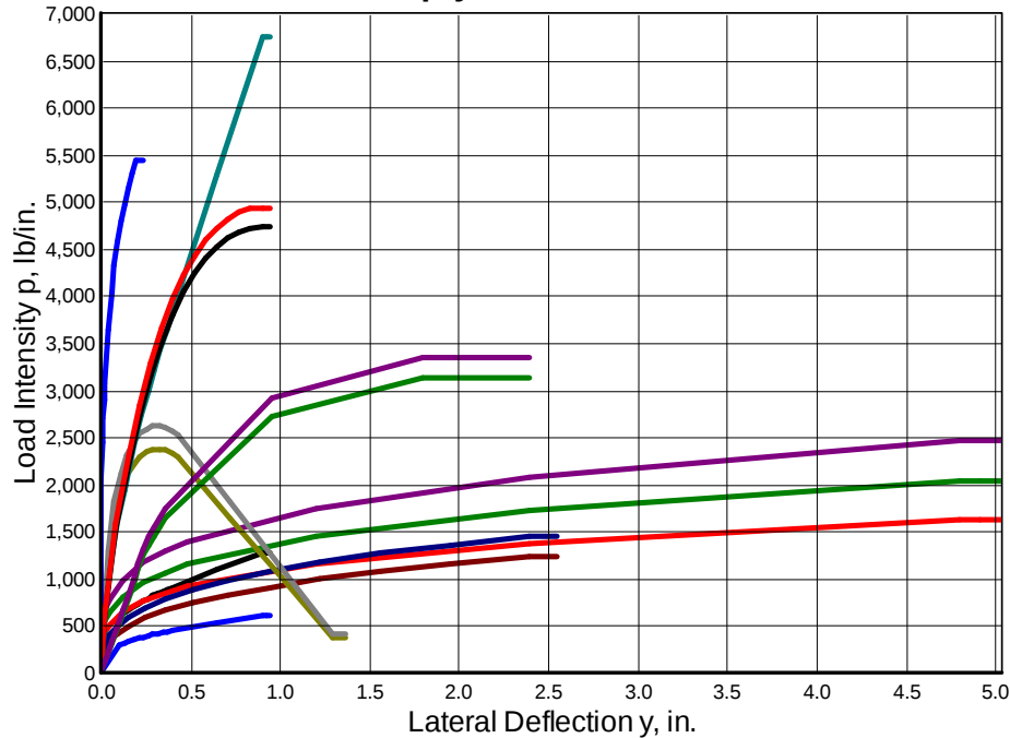
Figure 5-55 Standard Output of 17-point p - y Curves for Example 23
