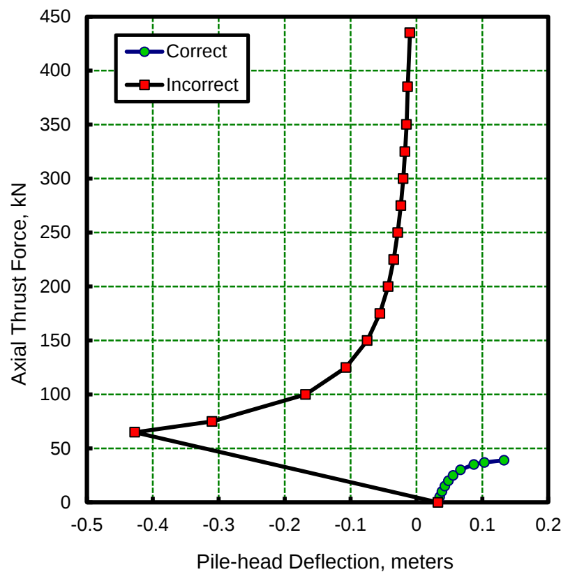
Figure 3-50 Example of Correct (blue) and Incorrect (black) Pile Buckling Analyses
