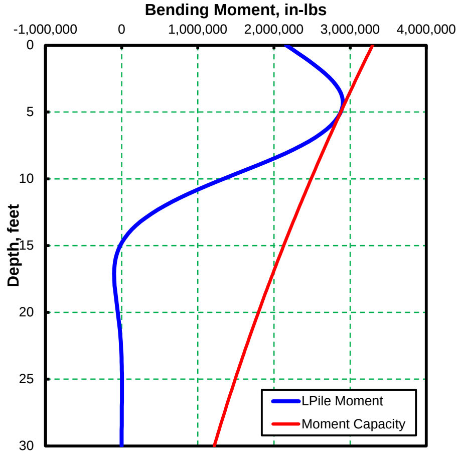
Figure 5-52 Bending Moment and Plastic Moment Capacity versus Depth for Example 22
