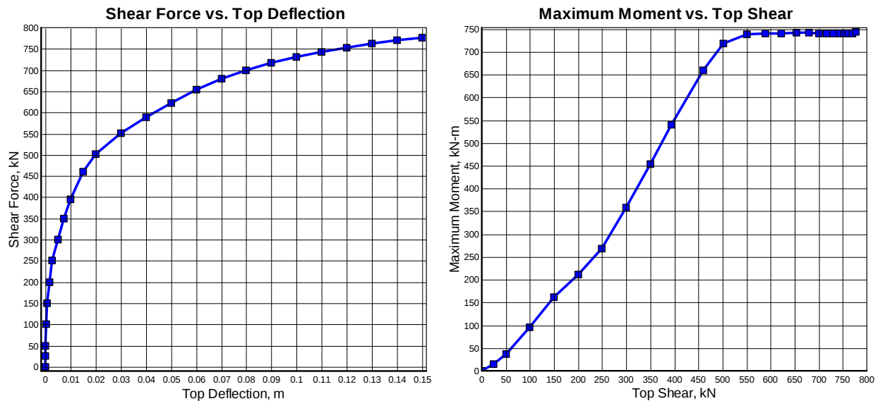
Figure 5-12 Shear Force versus Top Deflection and Maximum Bending Moment versus Top Shear Load for Fixed-head Conditions in Example 2c.
