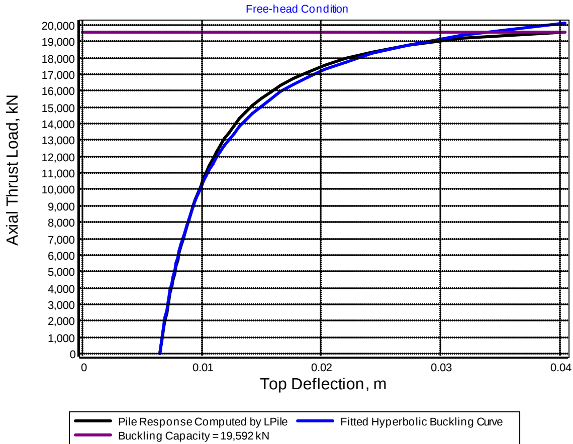
Figure 5-21 Results from LPILE Solution for Buckling Analysis, Example 4
