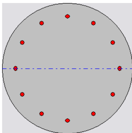
Figure 5-7 Cross-section of Drilled Shaft for Example 2.
