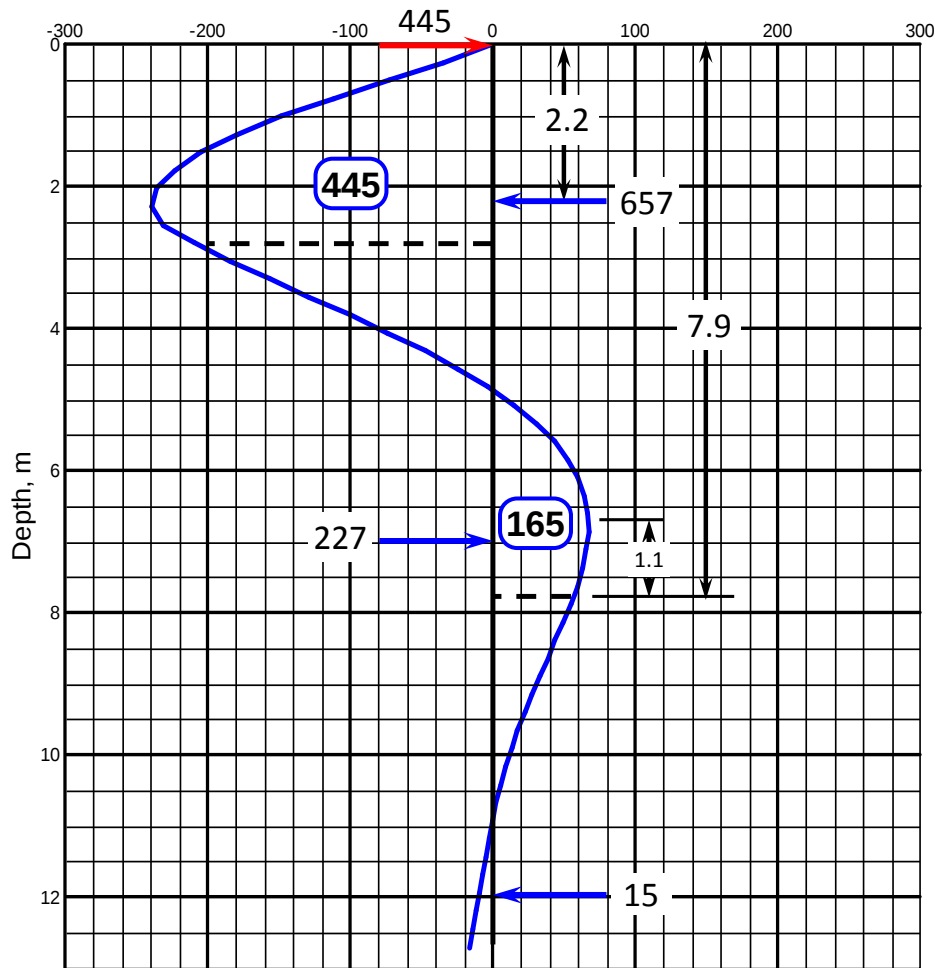
Figure 6-4 Plot of Mobilized Soil Resistance versus Depth
