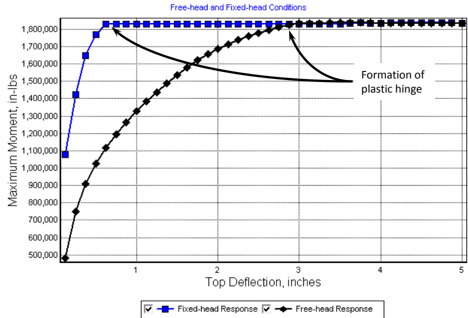
Figure 3-44 Maximum Moment in Pile versus Displacement from Pushover Analysis
