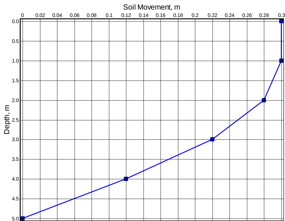
Figure 5-40 Lateral Spread Profile versus Depth for Example 12
