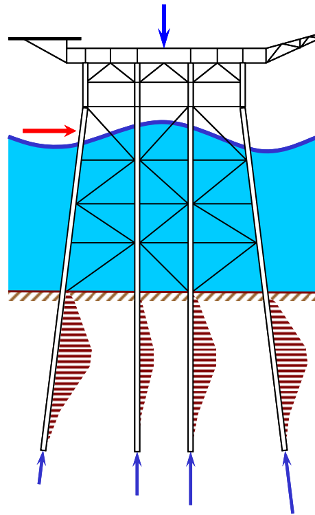
Figure 5-15 Idealized View of an Offshore Platform Subjected to Wave Loading, Example 3
