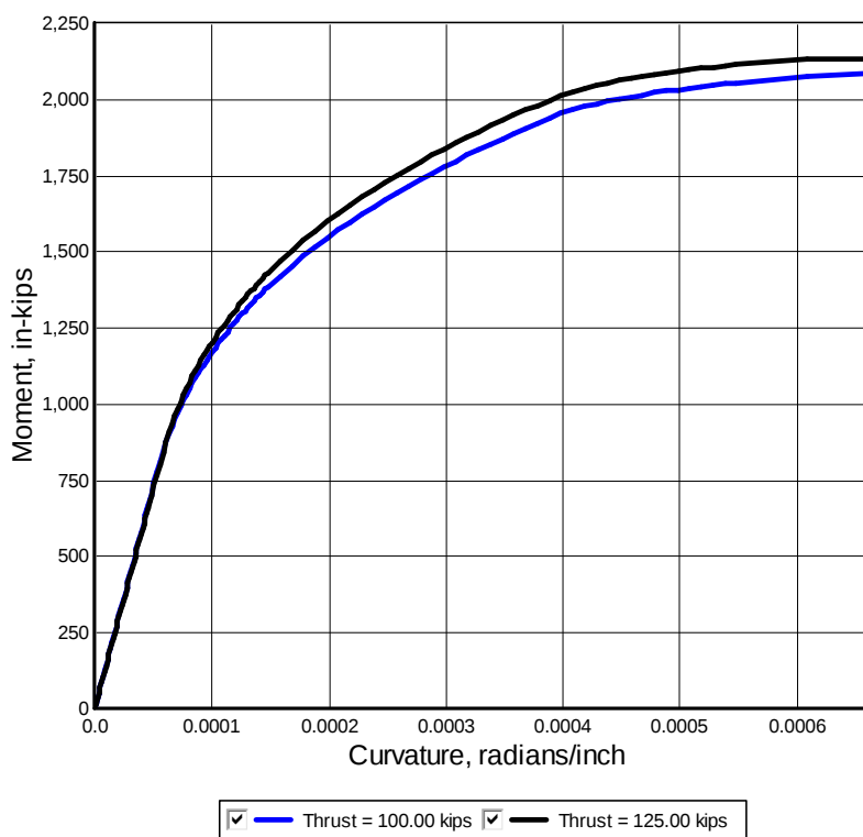
Figure 5-45 Moment versus Curvature of Prestressed Pile for Example 14
