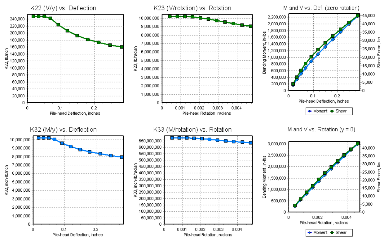
Figure 5-25 Stiffness Matrix Components versus Displacement and Rotation, Example 6
