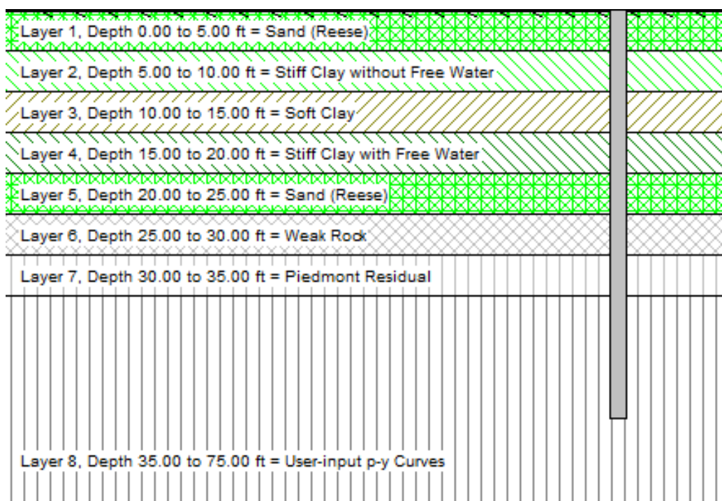
Figure 5-54 Pile and Soil Profile for Example 23
