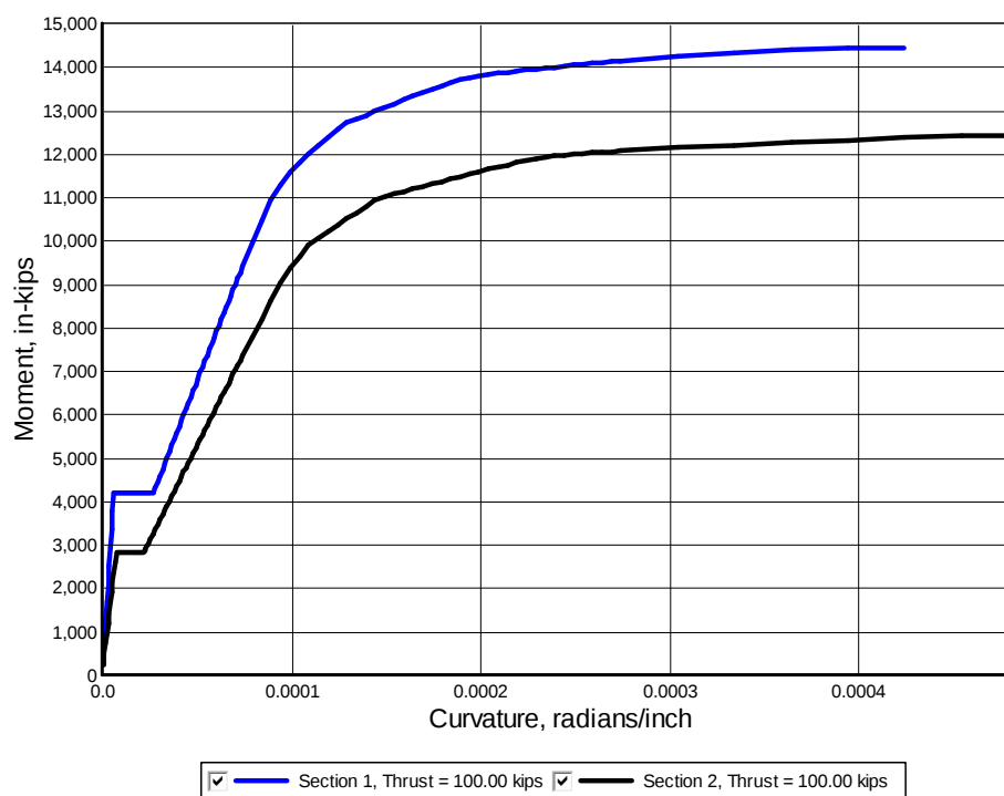
Figure 5-48 Moment versus Curvature for Dual Section Drilled Shaft of Example 17
