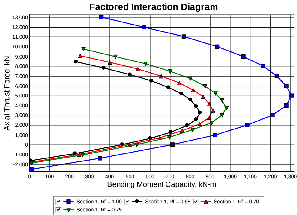
Figure 5-8 Factored Interaction Diagram for Example 2a.
