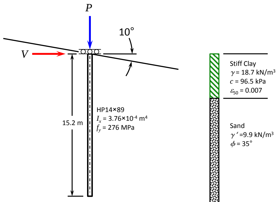
Figure 5-1 General Description of Example 1
