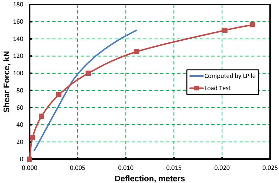
Figure 5-30 Comparison between Measured and Predicted Pile-head Load versus Deflection Curves for the 5-m Pile of Example 8
