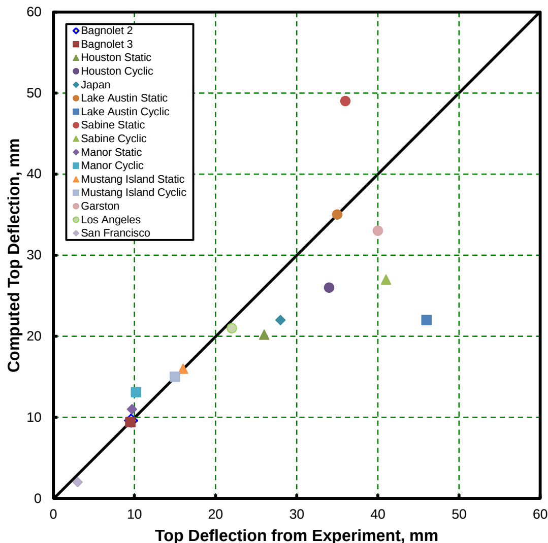
Figure 6-2 Comparison of Experimental and Computed Pile-head Deflections at Service Load
