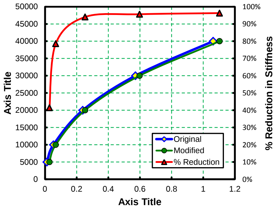
Figure 5-42 Pile-head Load versus Deflection Curves Using Original and Modified p - y Curves for Stiff Clay without Free Water and Percentage Reduction in Stiffness for Example 13
