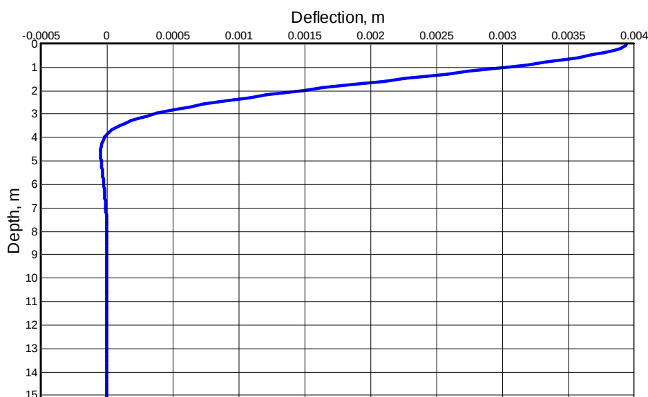
Figure 5-5 Curve of Deflection versus Depth for Example 1, Second Analysis
