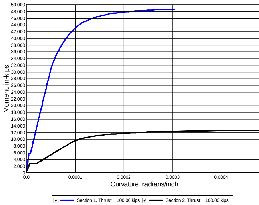
Figure 5-49 Moment versus Curvature for Dual Section Drilled Shaft with Permanent Casing of Example 18
