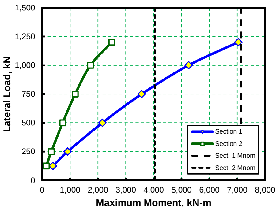
Figure 5-18 Results of Initial Computation with p - y Curves, Example 3
