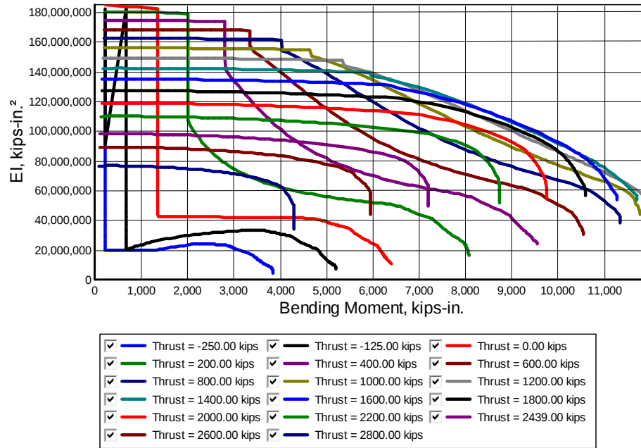
Figure 5-23 Bending Stiffness versus Bending Moment, Example 5
