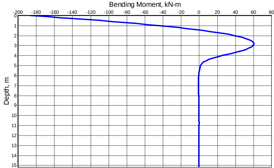
Figure 5-6 Bending Moment versus Depth for Example 1, Second Analysis
