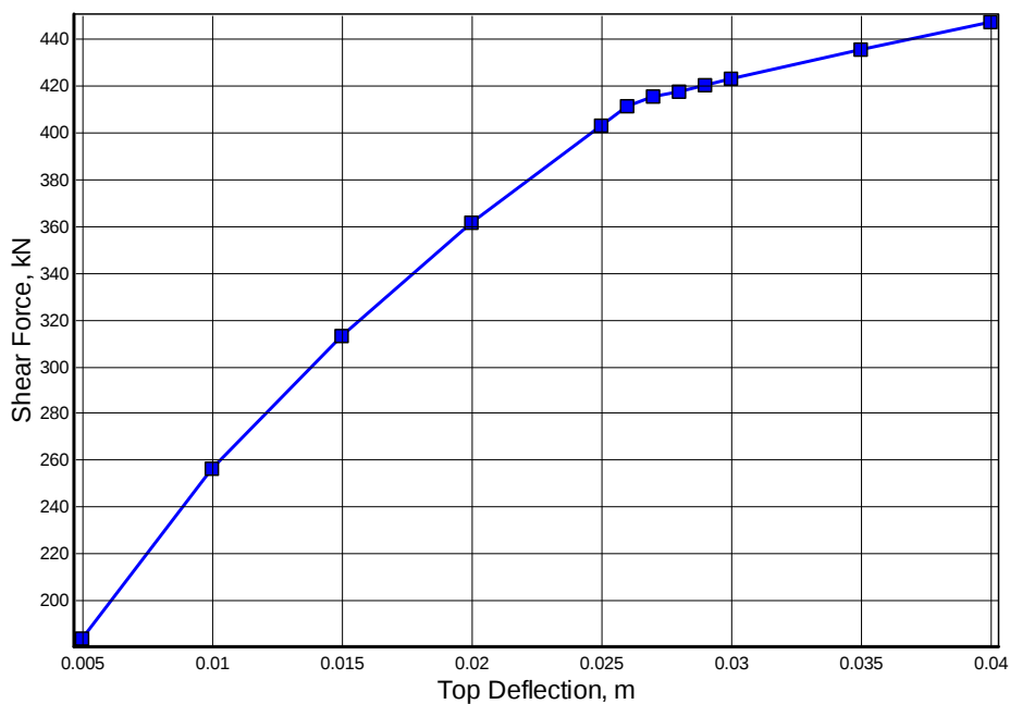
Figure 5-4 Generated Curve of Lateral Load versus Top Deflection for Example 1.
