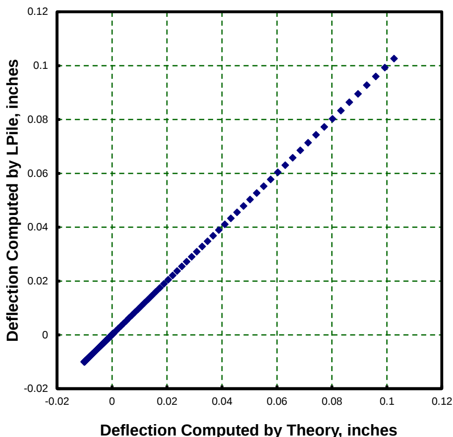
Figure 6-5 Verification of Pile Deflections
