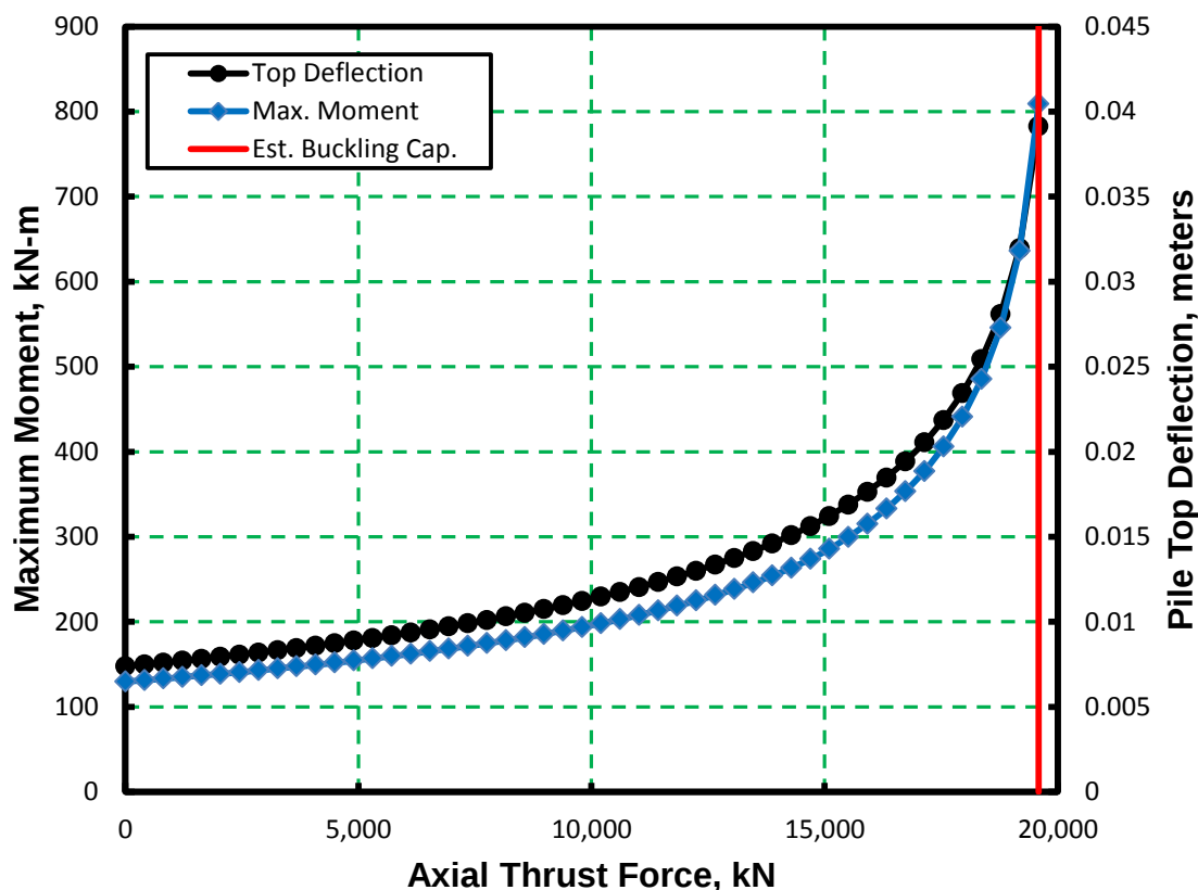
Figure 5-20 Pile-head Deflection and Maximum Bending Moment versus Axial Thrust Loading
