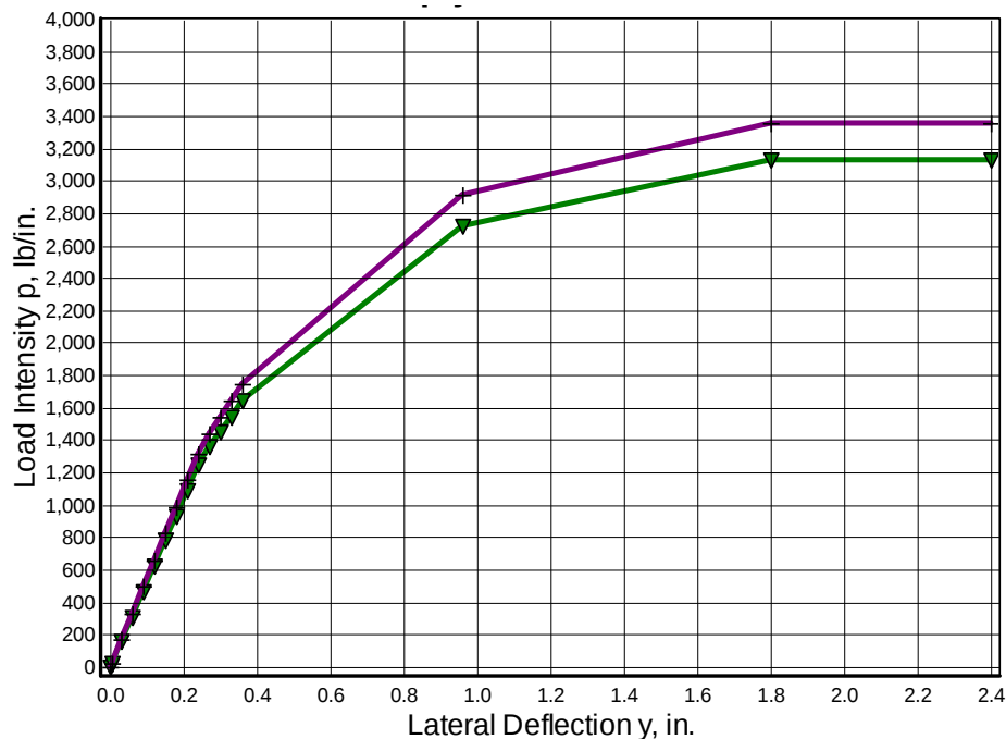
Figure 5-56 User-input p - y Curves Interpolated with Depth Using 17 Points for Example 23
