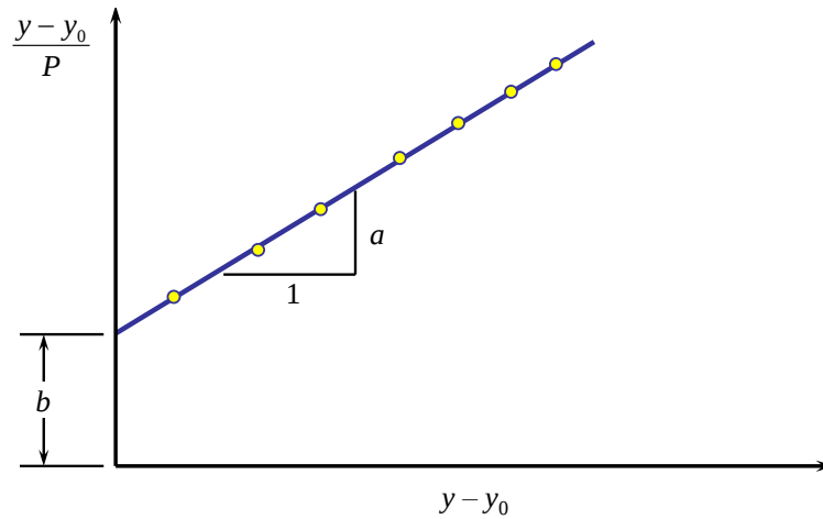
Figure 3-48 Redrawn Pile Buckling Results Used for Curve Fitting
