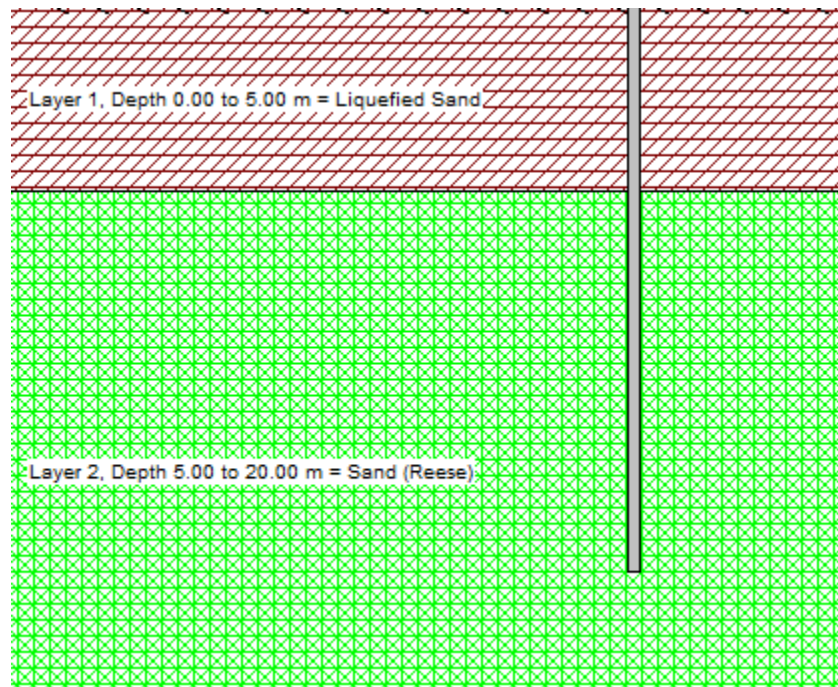
Figure 5-39 Pile and Soil Profile for Example 12
