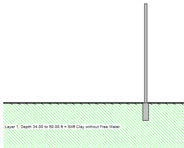
Figure 5-51 Pile and Soil Profile for Embedded Pole of Example 20
