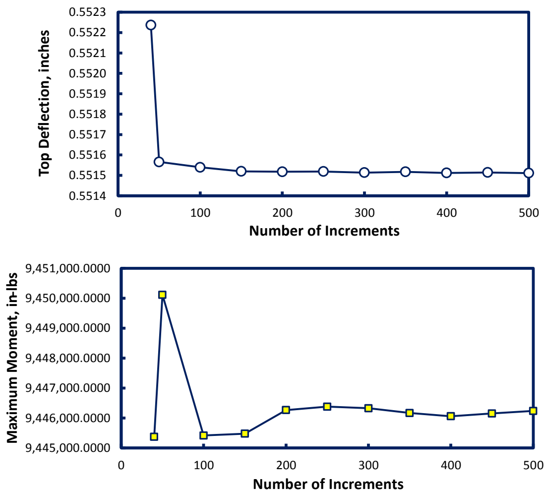
Figure 6-3 Influence of Increment Length on Computed Values of Pile-head Deflection and Maximum Bending Moment
