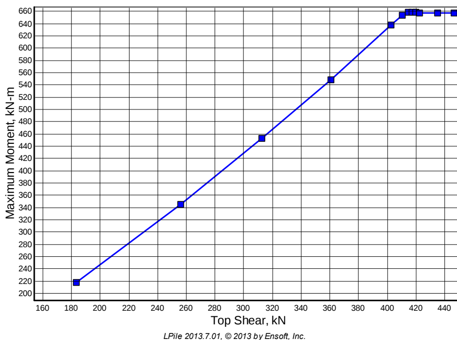
Figure 5-3 Generated Curve of Lateral Load versus Maximum Moment for Example 1.
