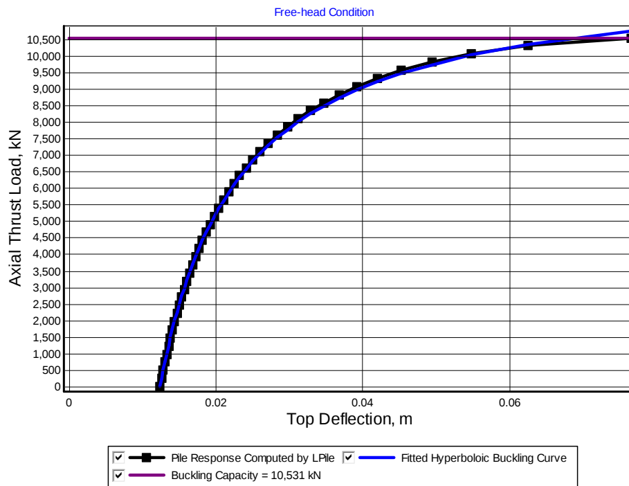
Figure 3-49 Results from Pile Buckling Analysis
