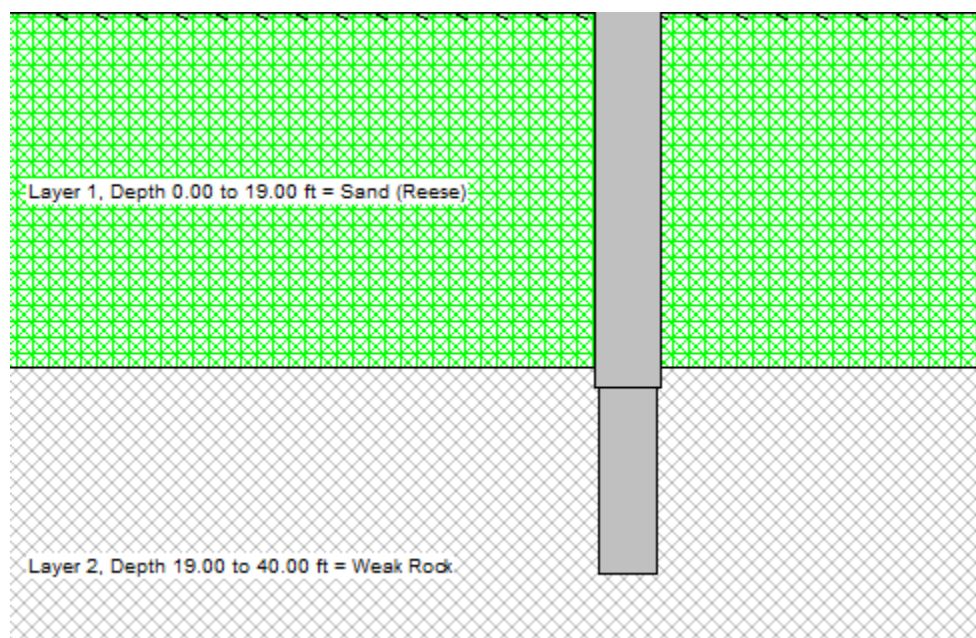
Figure 5-47 Pile and Soil Profile for Example 17
