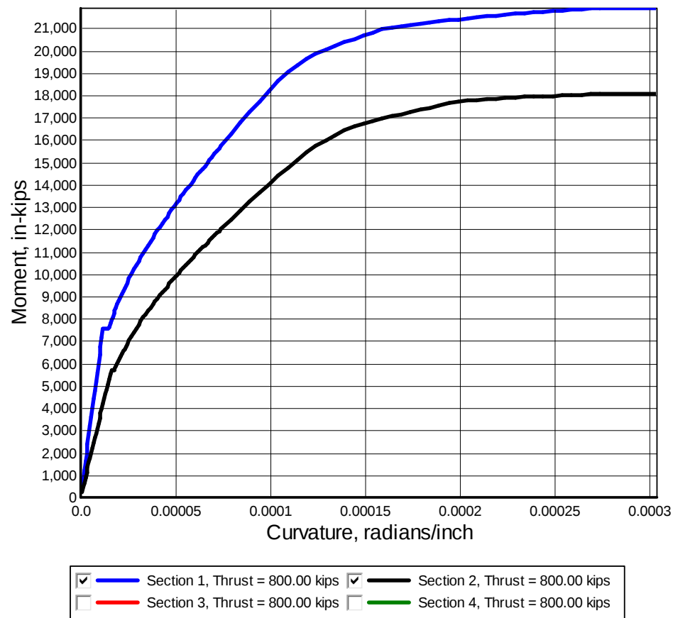
Figure 5-33 Moment versus Curvature for Sections 1 and 2, Example 9
