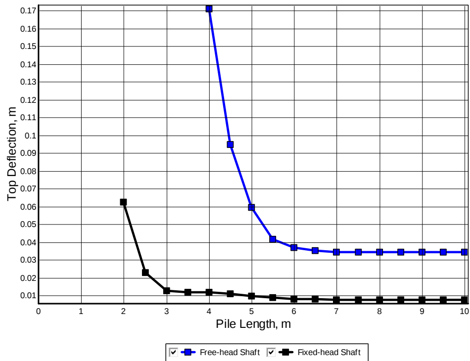
Figure 5-14 Top Deflection versus Pile Length for Example 2d
