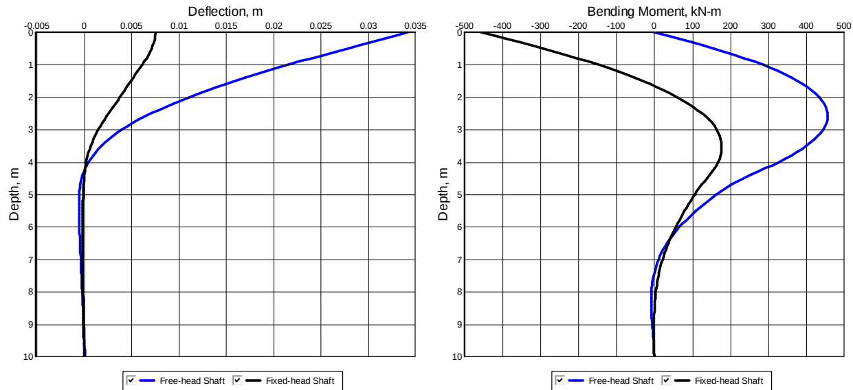
Figure 5-13 Results for Free-head and Fixed-head Loading Conditions for Example 2d
