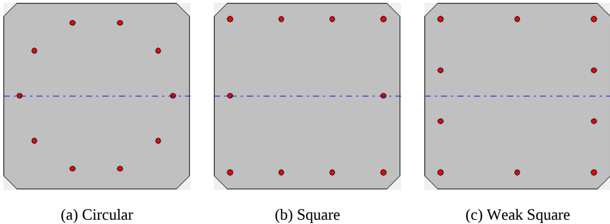
Figure 3-21 Automatic Prestressing Arrangements for Square Prestressed Piles
