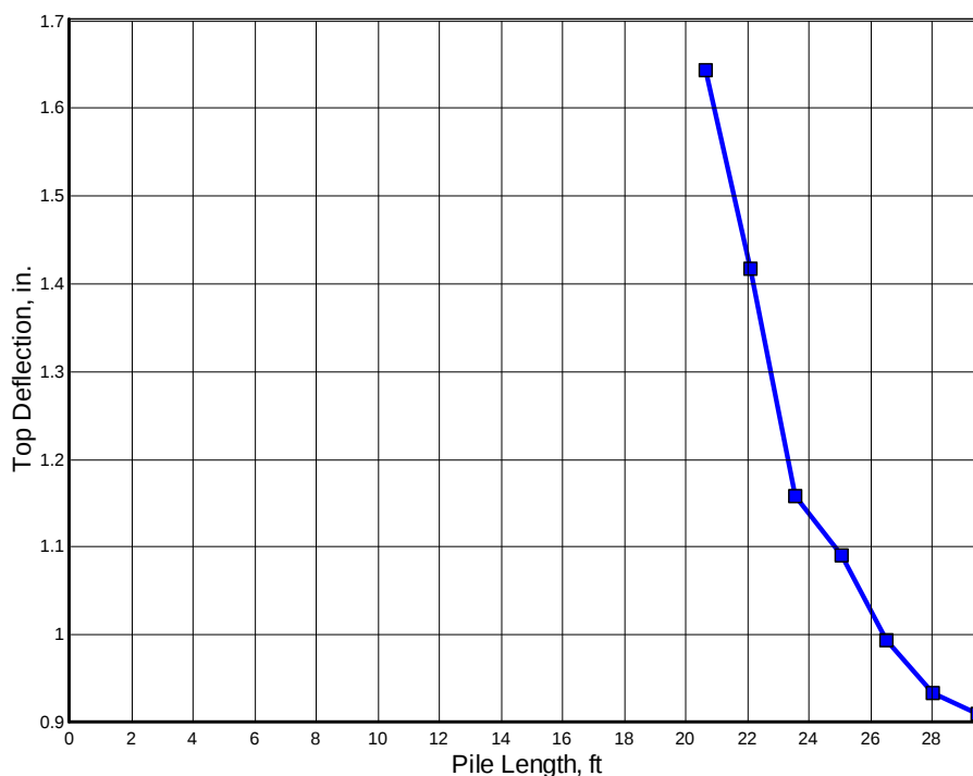
Figure 5-35 Top Deflection versus Pile Length, Example 9
