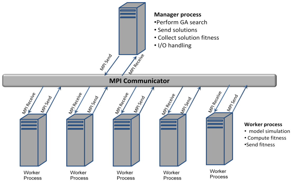
Figure 7.5 Manager-worker Parallel Computation Model
