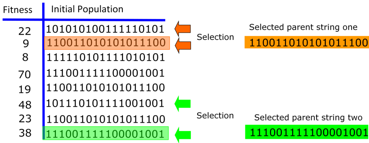
Figure 7.2 Example GA population solutions and selection operation
