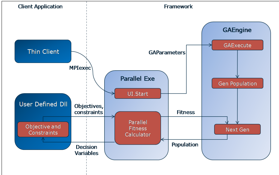
Figure 7.6 Architecture overview of parallel optimization framework
