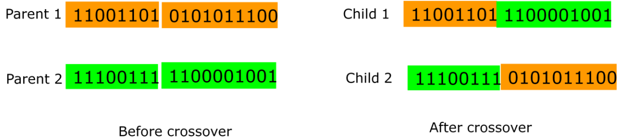
Figure 7.3 Genetic algorithm crossover operations
