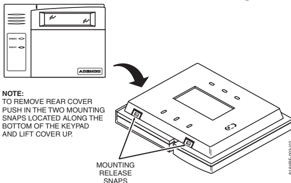
Figure 1. Removing the Case Back
