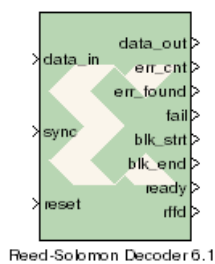
Reed-Solomon Decoder 6.1
