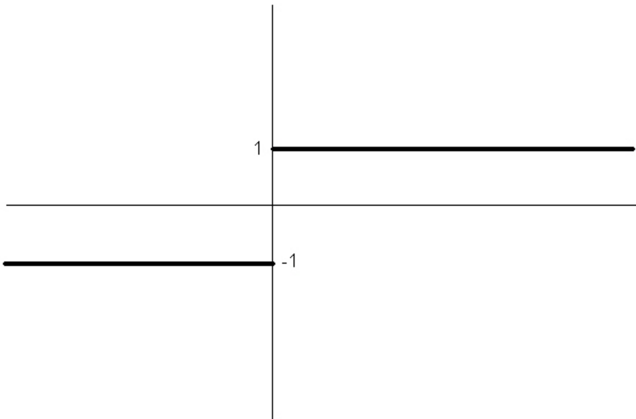
Figure 2. The discontinuous piecewise-linear function sign()
