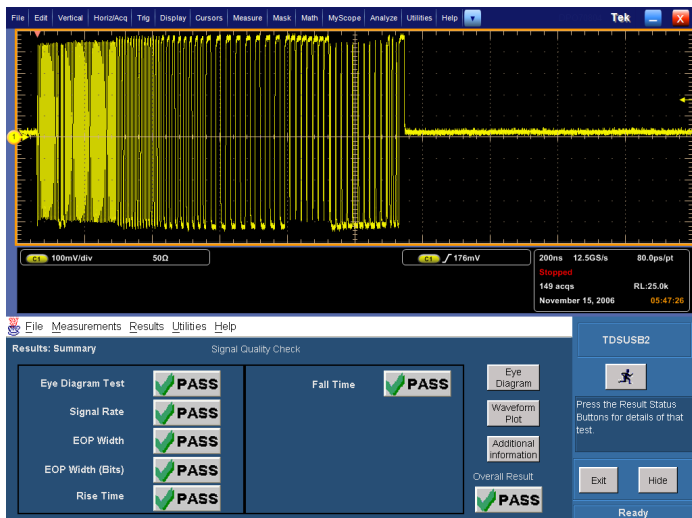
TDSUSB2 compliance test results.
