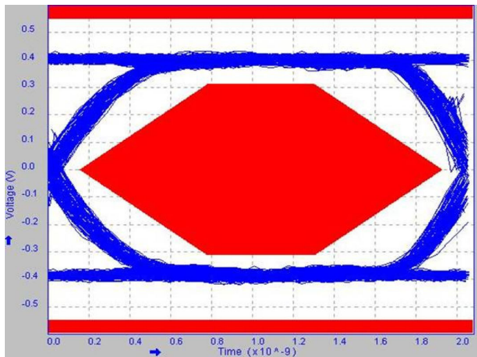
TDSUSB2 Automated USB eye diagram analysis.
