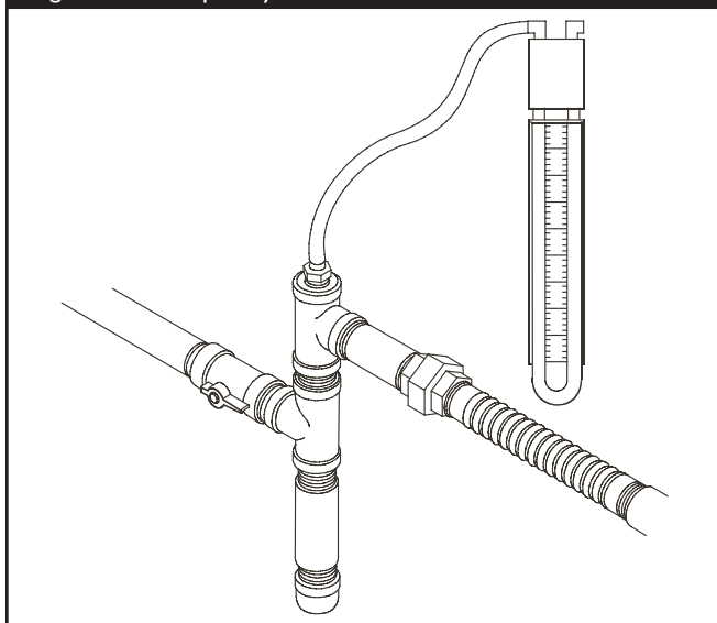
Figure 5 — Temporary Manometer Installed
