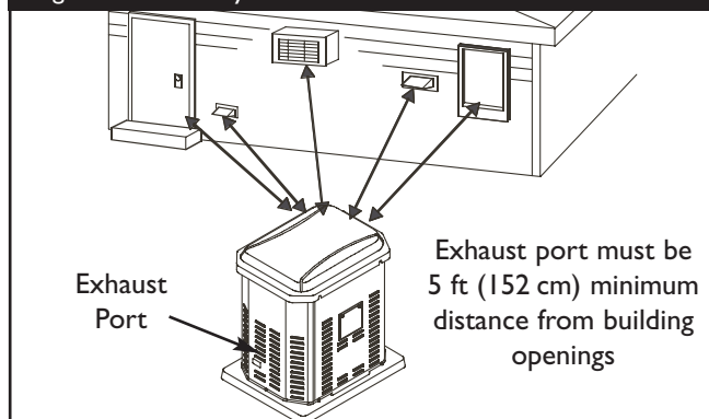
Figure 1 — Standby Generator Clearances
