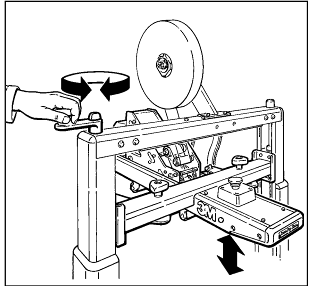
Figure 3-2 – Upper Taping Head
