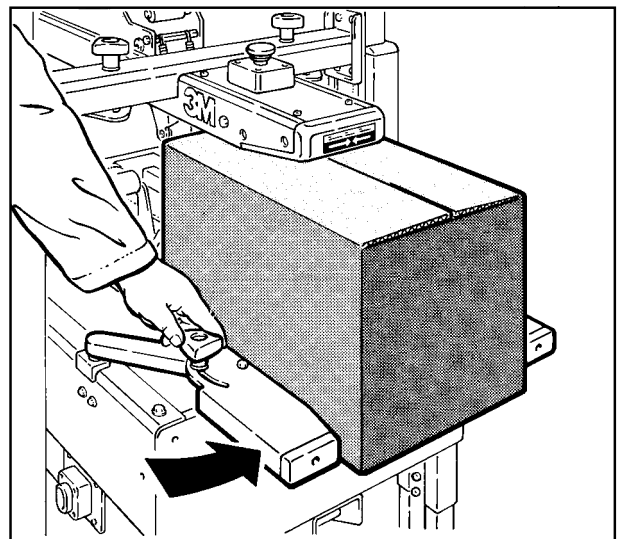
Figure 3-4 – Side Guides
