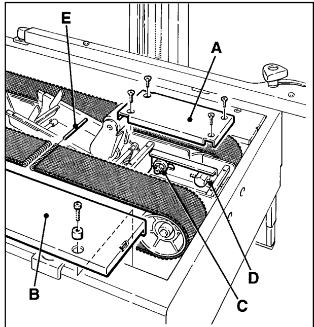
Figure 4-2 – Box Drive Belt Replacement
