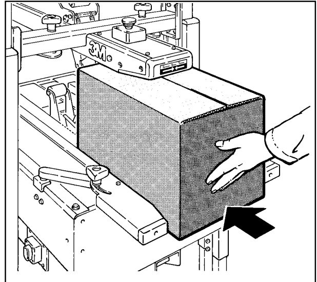
Figure 3-5 – Check Adjustments
