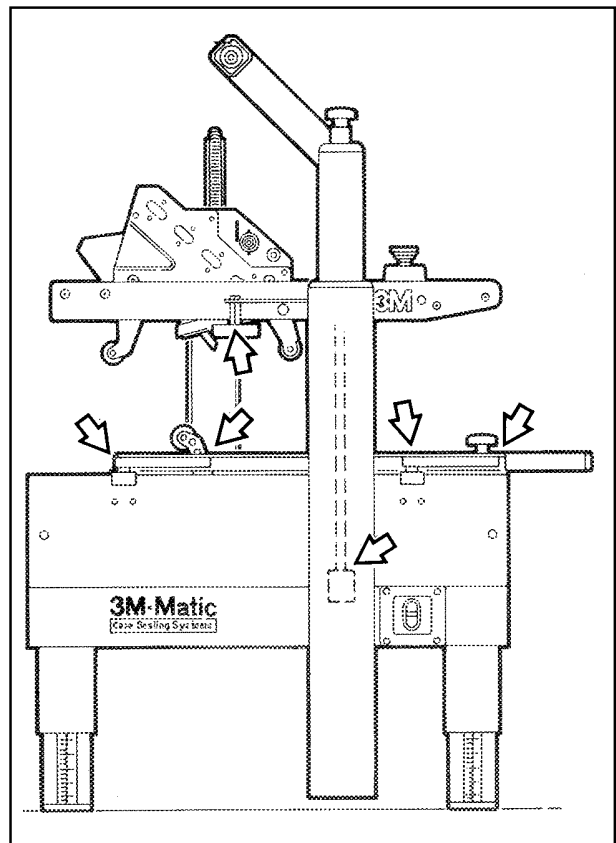
Figure 4-1 – Lubrication Points – Frame
