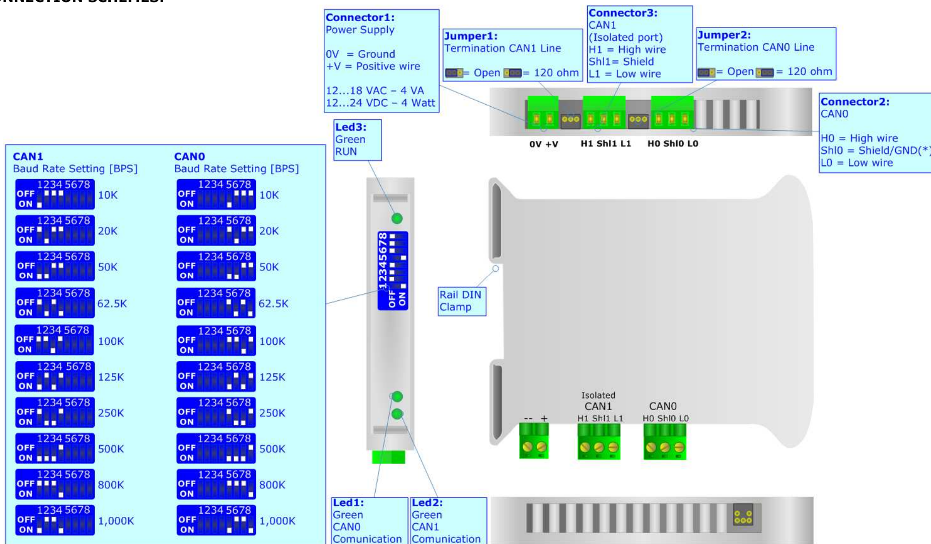
Figure 1: Connection scheme for HD67180
