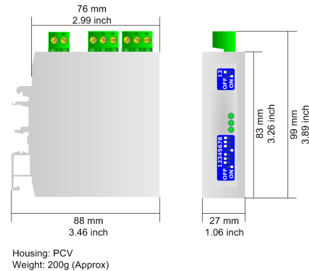
Figure 8: Mechanical dimensions scheme for HD67180R
