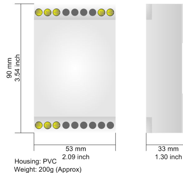
Figure 6: Mechanical dimensions scheme for HD67180M
