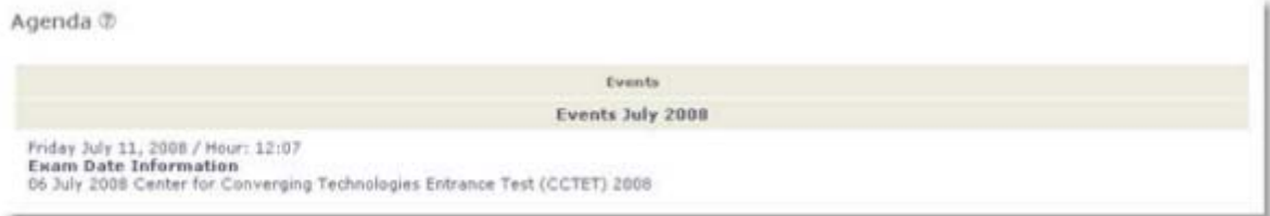
Pic. 14. Agenda
