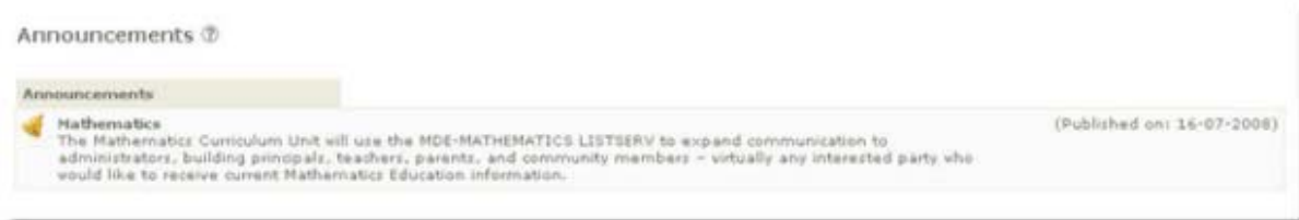
Pic. 15. Announcements
