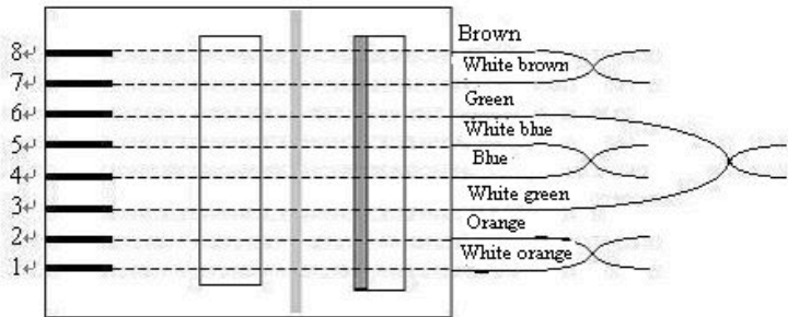
RJ45 Connector TIA/EIA-568B Criterion
