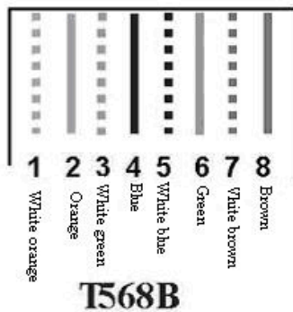
RJ45 Connector TIA/EIA-568B Criterion
