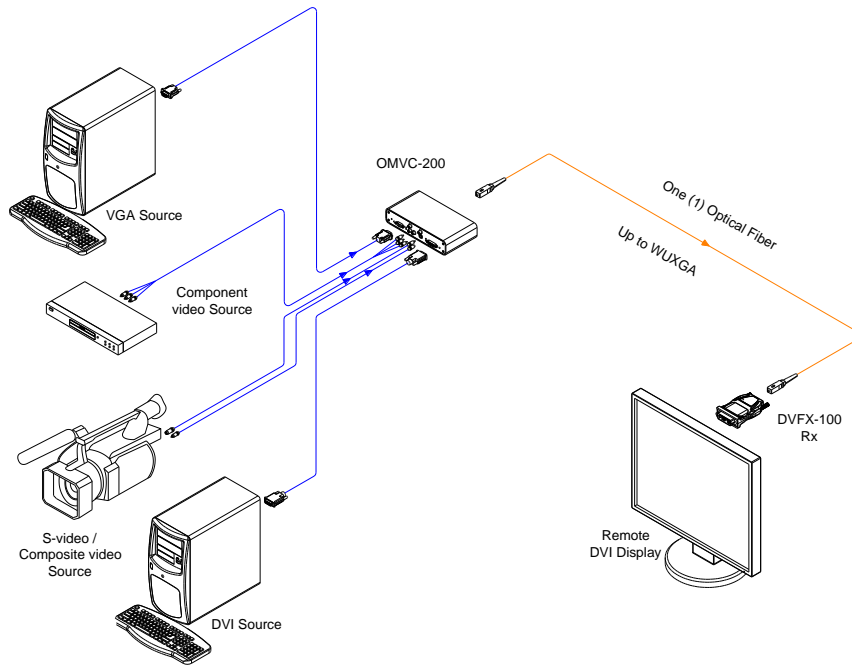
Figure 1 – Connection Diagram of OMVC-200
