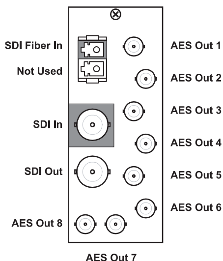
Figure 2.4 Cable Designations for the 8320AR-048A Rear Module
