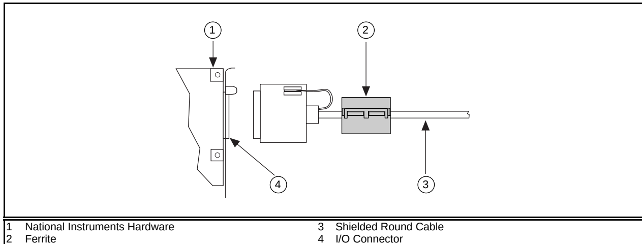
Figure 3. Ferrite Installation for an Instrumentation System with a Shielded Round Cable
