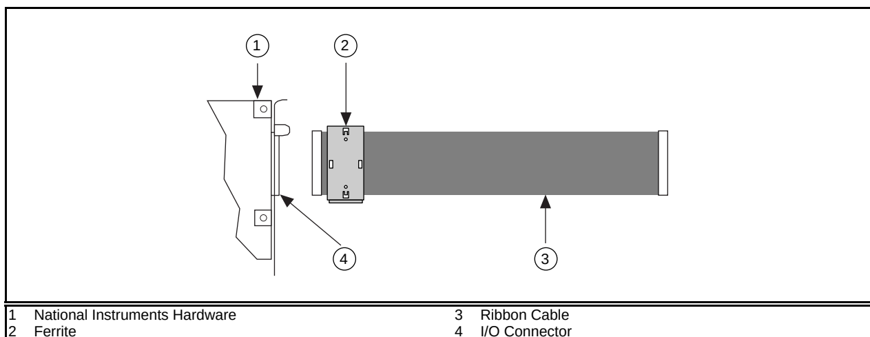
Figure 2. Ferrite Installation for an Instrumentation System with a Ribbon Cable
