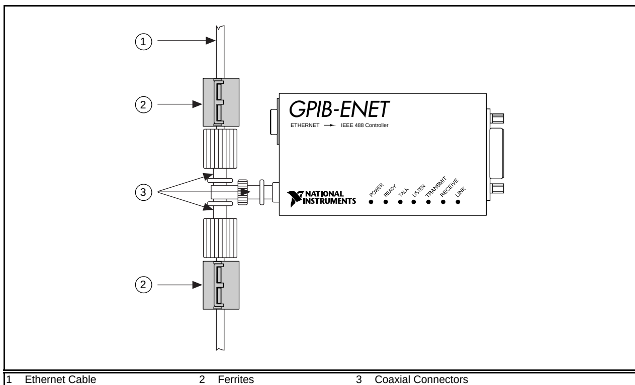
Figure 4. Ferrites Installed on the GPIB-ENET Ethernet Cables
