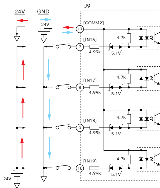
[IN6~9,16~19] SIGNALS
