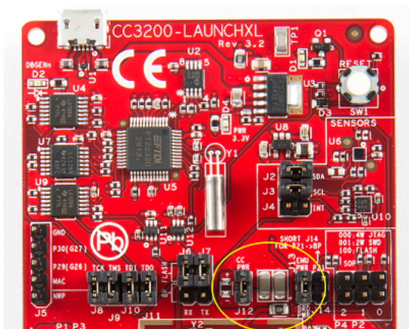
Figure 9. Powering From USB
