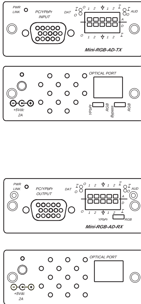
Figure 1-1 Mini-RGB-AD Front and Rear Panels
