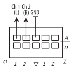
Figure 2-3b Audio terminal block pinout for audio output for Mini-RGB-AD.
