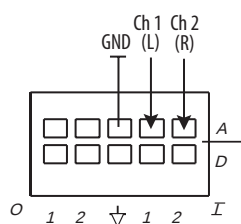
Figure 2-3a Audio terminal block pinout for audio input to Mini-RGB-AD.
