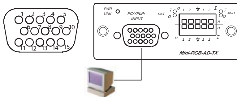
Figure 2-2 Electrical Connection
