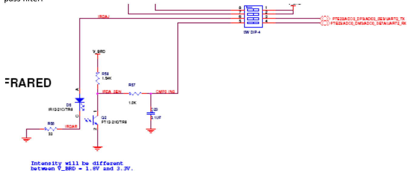
Figure 3 Infrared circuit
